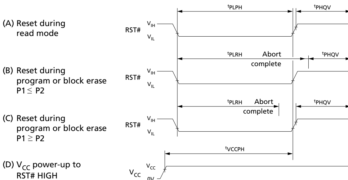
Figure 23: Reset Operation Waveforms
