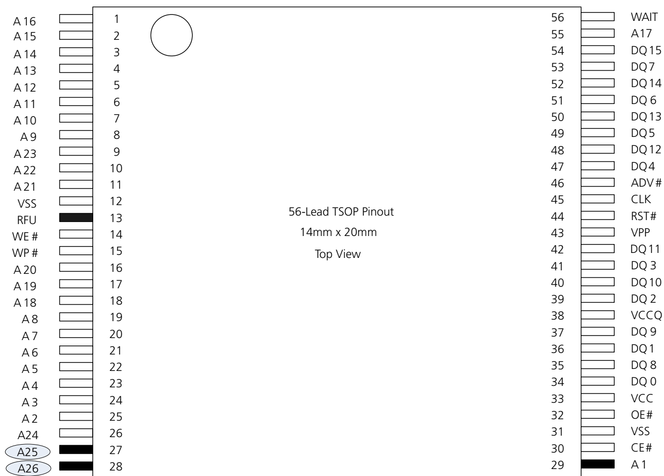
Figure 6: 56-Lead TSOP Pinout – 512Mb and 1Gb
