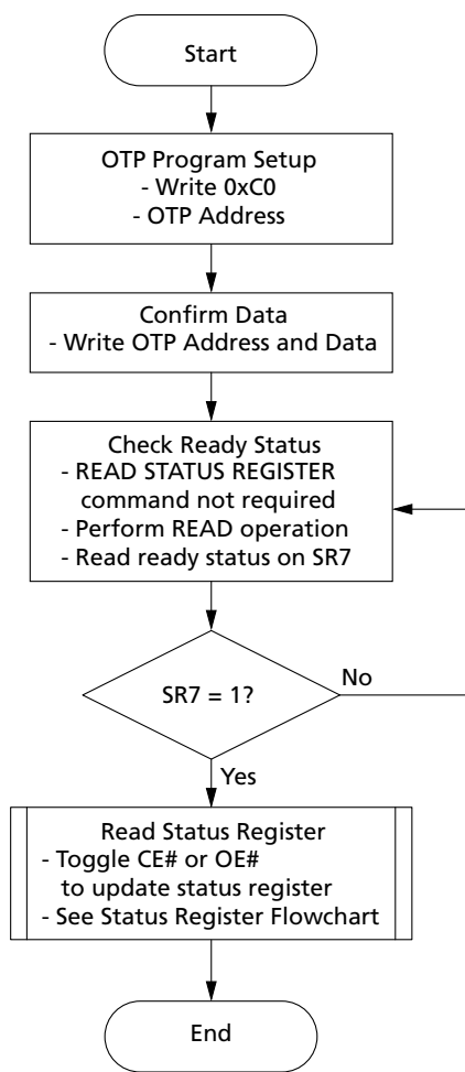
Figure 21: OTP Register Programming Procedure
