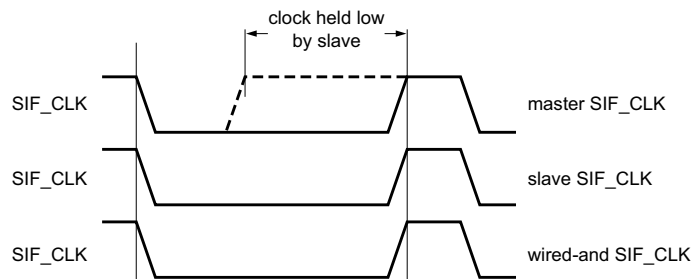
Fig 36. Clock stretching
