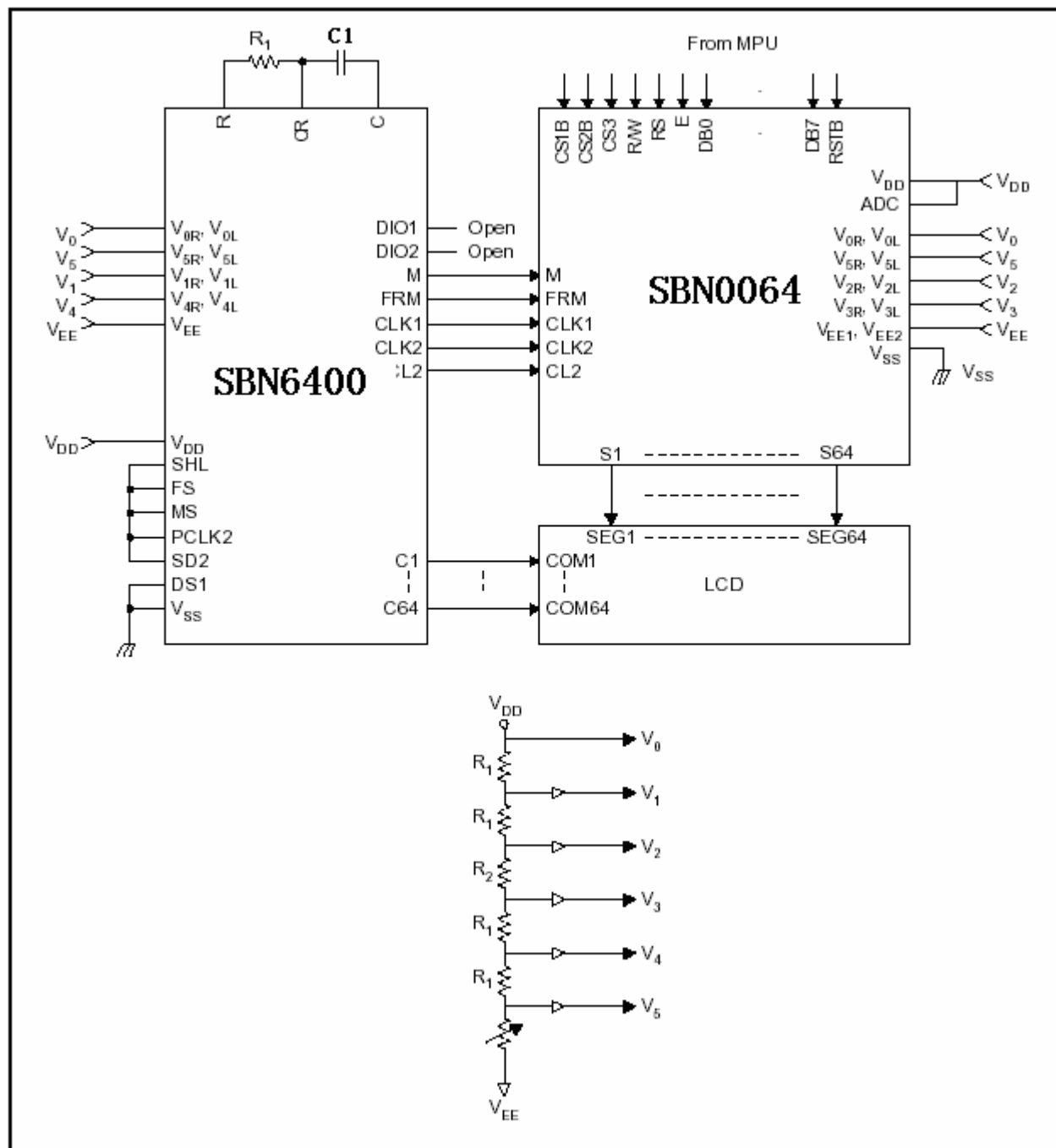
1/64 DUTY COMMON DRIVER (SBN6400) NTERFACE CIRCUIT
