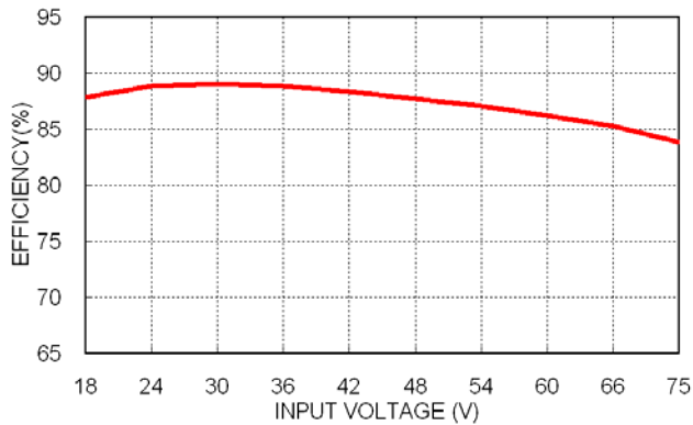
JFCW48S5-3000 Efficiency vs. Input Voltage
