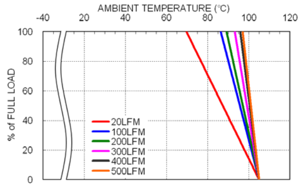
JFCW48S5-3000 Derating Curve with Heat-Sink
