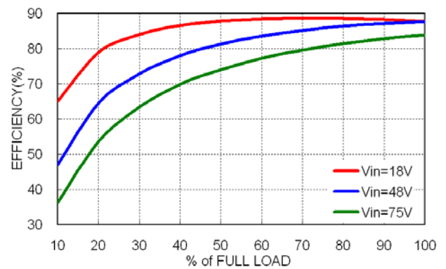
JFCW48S5-3000 Efficiency vs. Output Load
