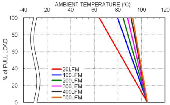
JFCW48S5-3000 Derating Curve
