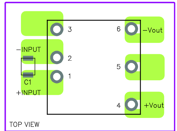
Recommended Layout with Input Filter
