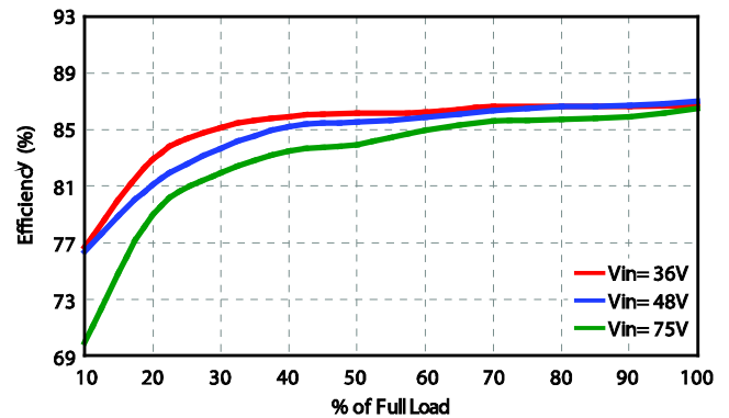
JFC48S05-10 Efficiency vs Output Load
