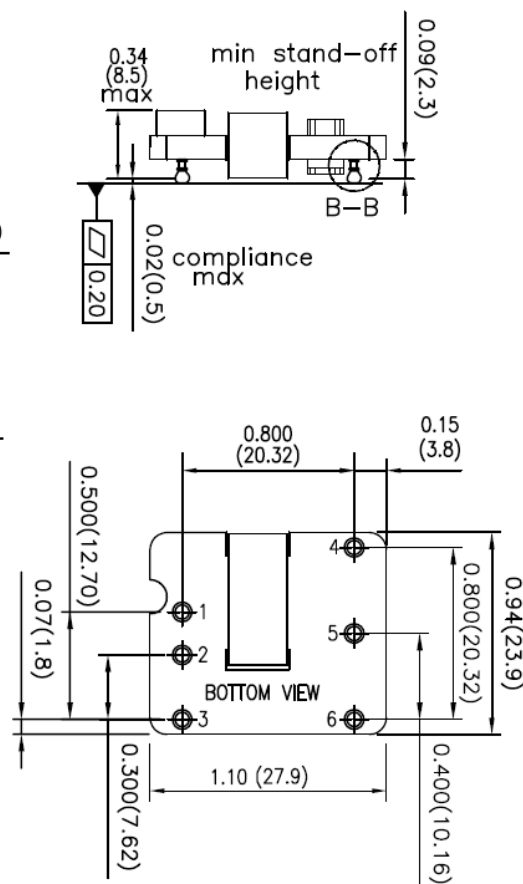
PAD LAYOUT 6 PADS \phi 2.8 mm
