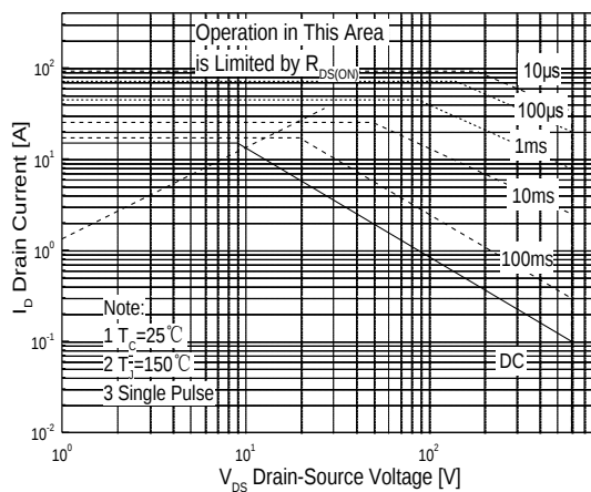
Maximum Safe Operating Area For JCS15N60FH
