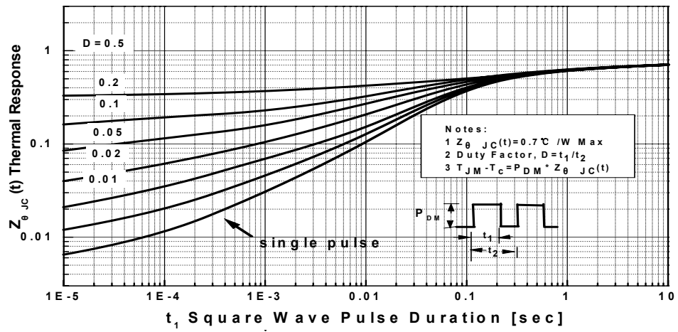
Transient Thermal Response Curve For JCS10N60BT
