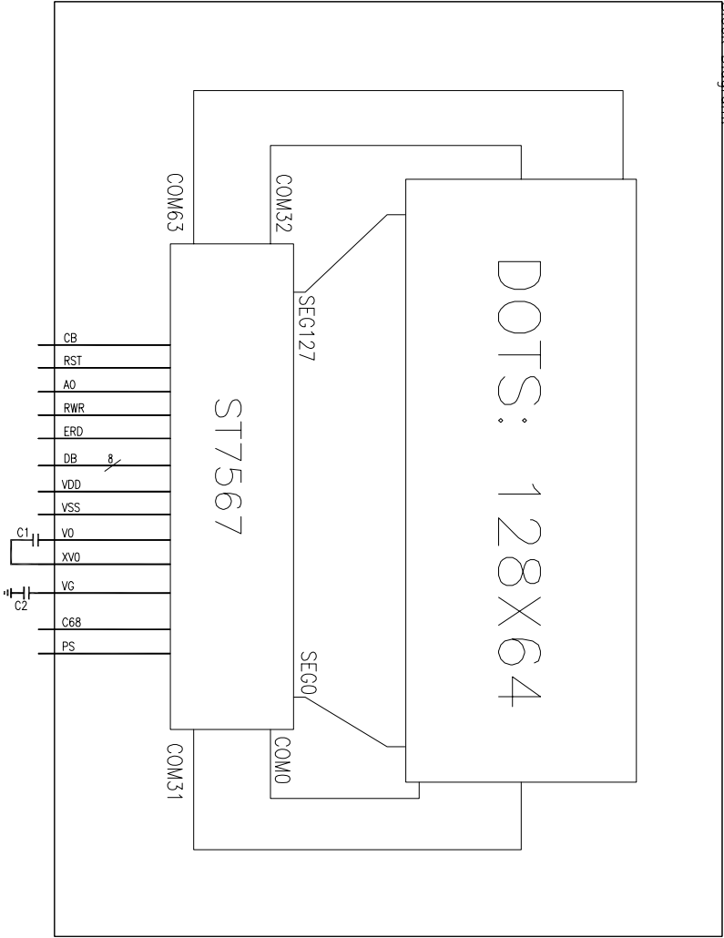
Block Diagram:
