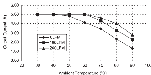
SMT Version Derating Curve for 3.3 VDC Output
