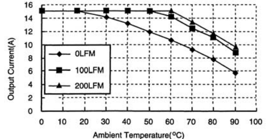
Derating Curve for 5.0 VDC Input
