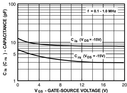
Figure 10. Capacitance vs. Voltage
