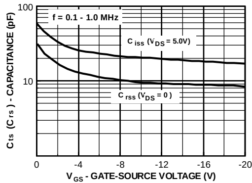
Common Drain-Source
