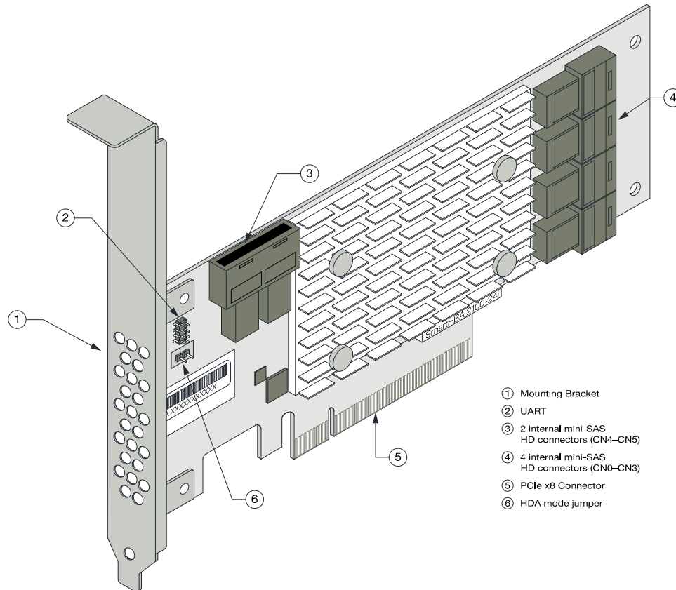
Figure 10 • Microsemi Adaptec SmartHBA 2100-24i Features
