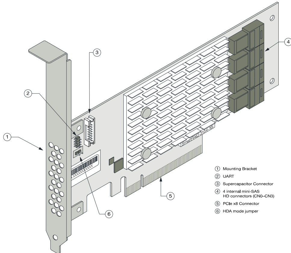
Figure 5 • Microsemi Adaptec SmartRAID 3154-16i
