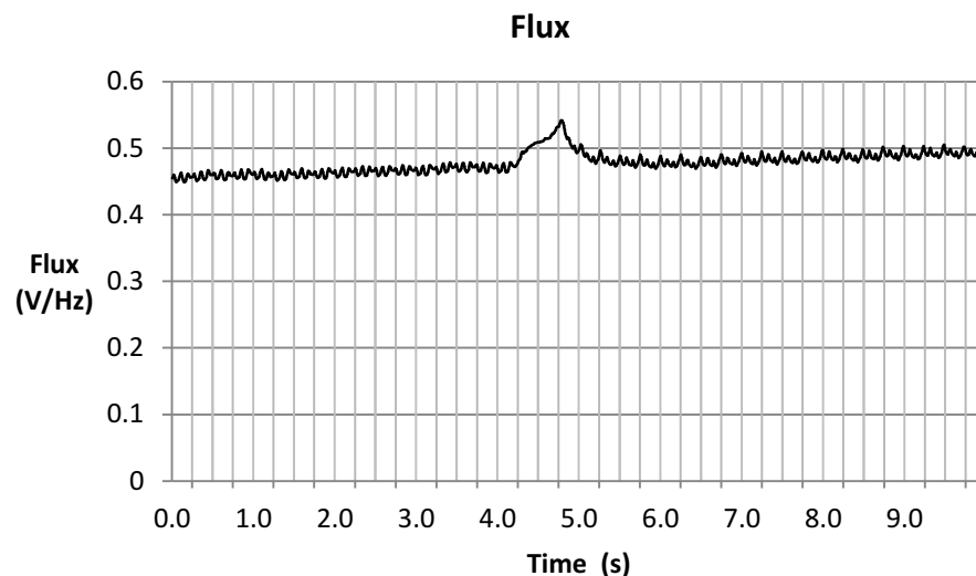
Figure 14-20. Flux Plot
