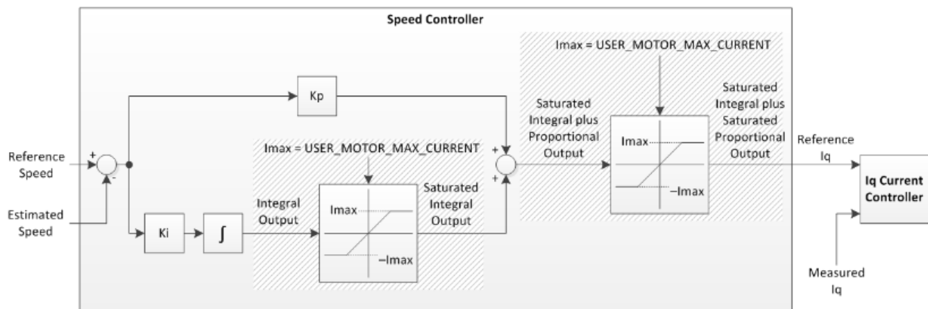
Figure 14-35. Speed Controller Cycle
