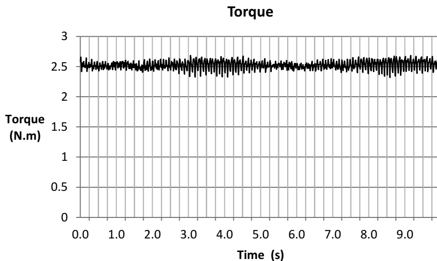
Figure 14-71. Torque Plot
