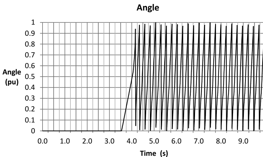
Figure 14-37. Angle Plot
