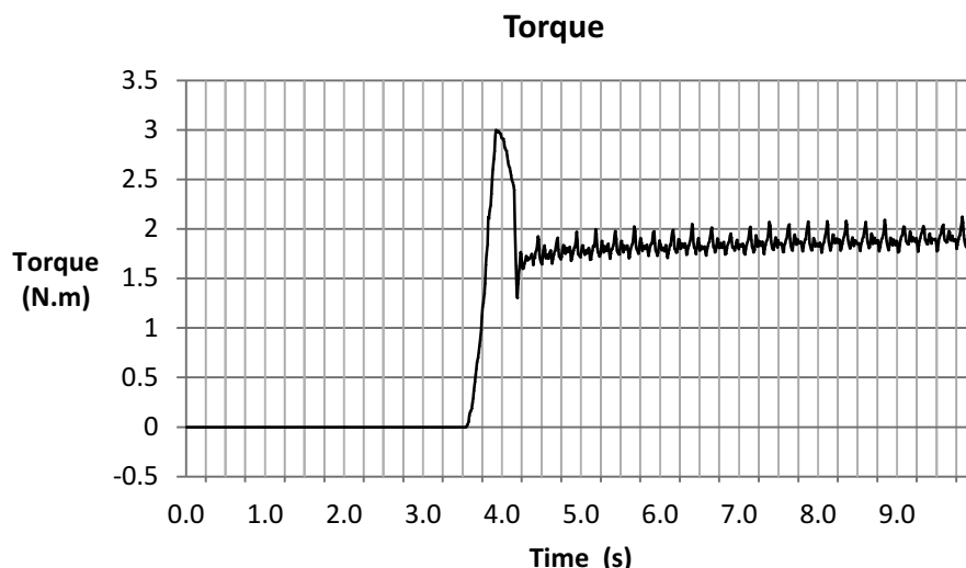
Figure 14-40. Torque Plot
