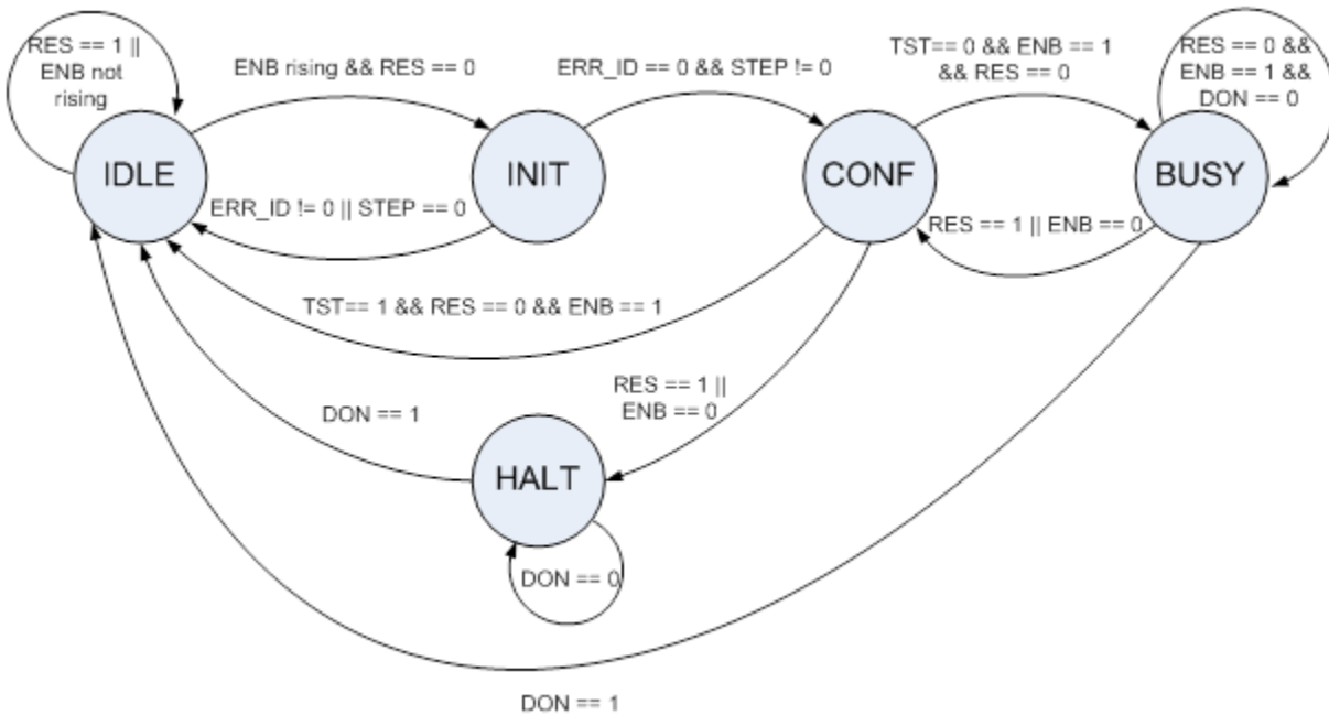
Figure 3-18. SpinTAC Position Move State Transition Map
