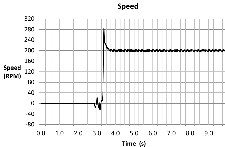
Figure 14-53. Speed Plot
