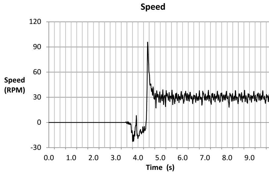
Figure 14-46. Speed Plot
