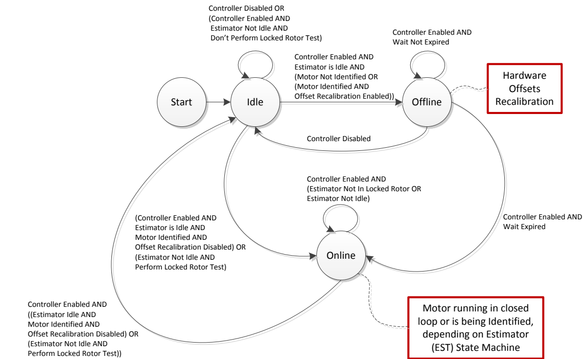
Figure 6-4. Controller (CTRL) State Diagram
