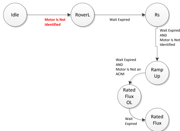
Figure 6-20. PMSM Rated Flux EST State
