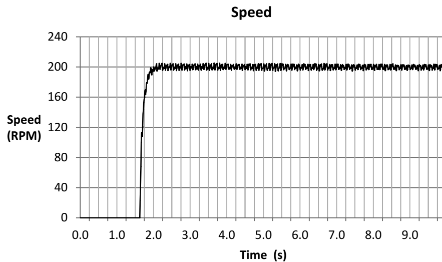
Figure 14-61. Speed Plot
