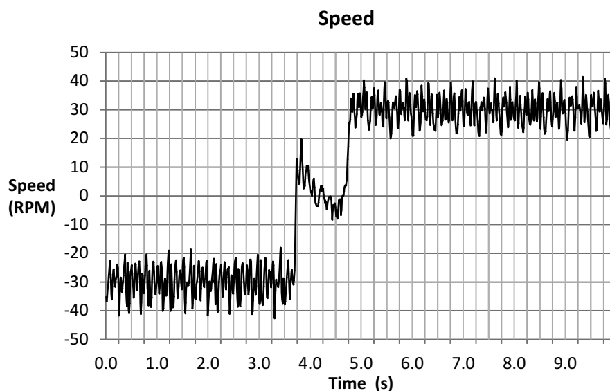
Figure 14-30. Speed Plot
