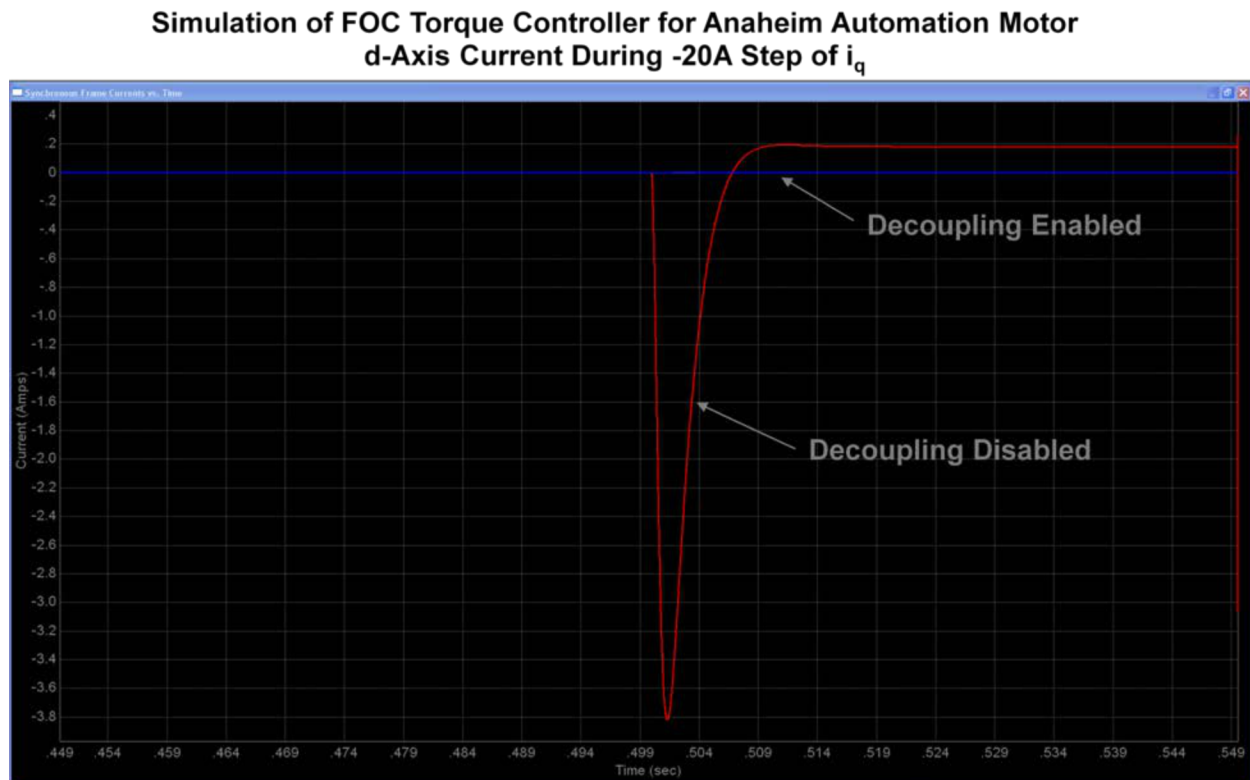
Figure 11-20. Simulated Effectiveness of Current Regulator Decoupling
