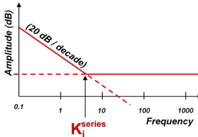
Figure 11-4. Frequency Response
