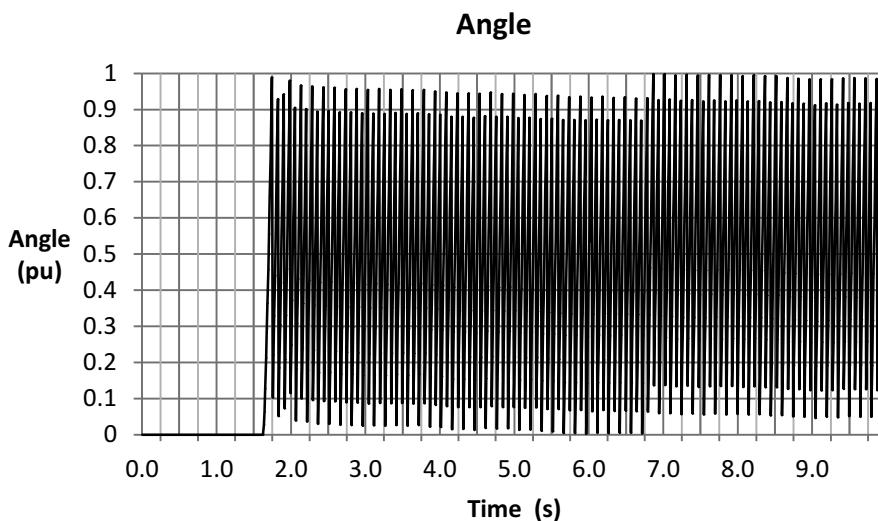
Figure 14-59. Angle Plot
