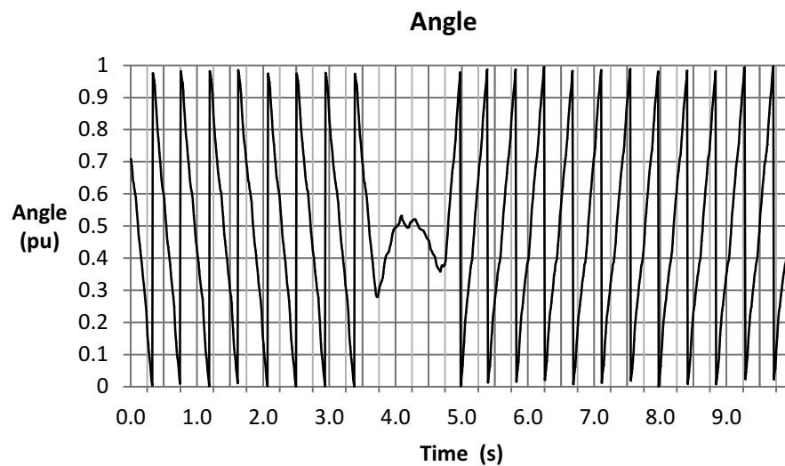
Figure 14-28. Angle Plot
