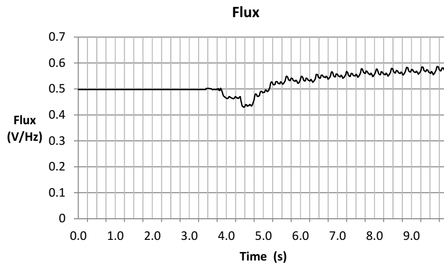
Figure 14-43. Flux Plot
