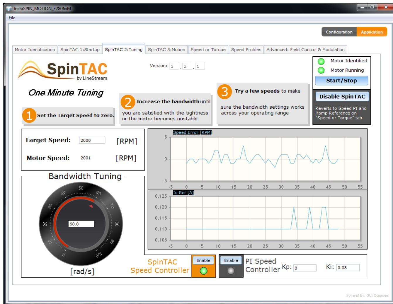
Figure 2-4. InstaSPIN-MOTION GUI SpinTAC 2:Tuning Tab
