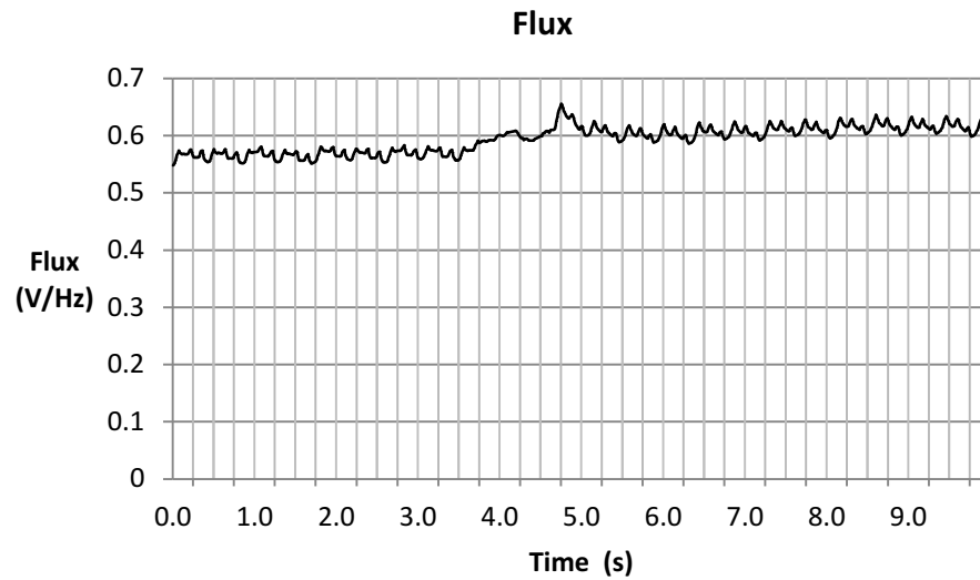
Figure 14-27. Flux Plot
