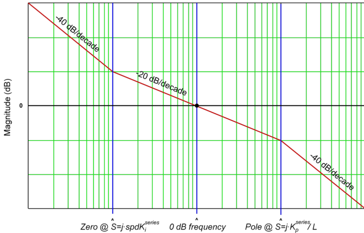
Figure 11-7. Bode Plot
