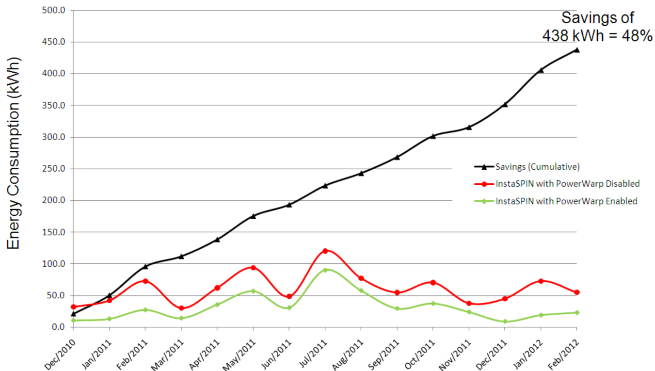
Figure 16-8. InstaSPIN-FOC with PowerWarp Enabled vs. InstaSPIN-FOC with PowerWarp Disabled
