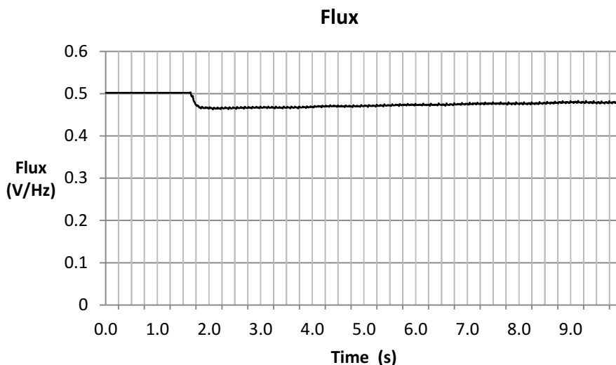
Figure 14-58. Flux Plot
