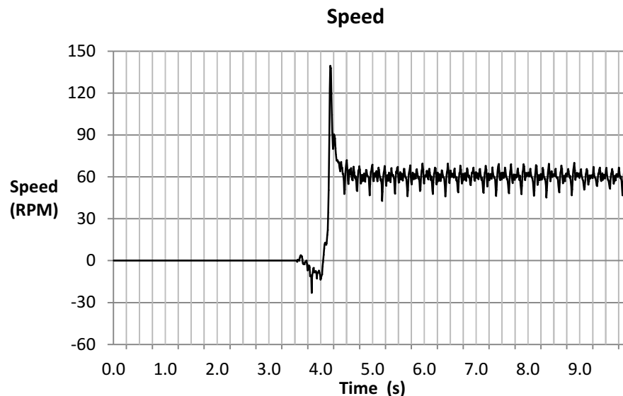
Figure 14-39. Speed Plot
