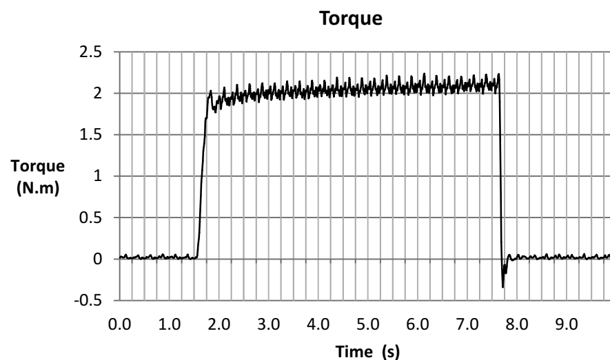
Figure 14-9. Torque Plot
