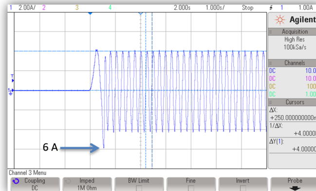
Figure 14-34. Standstill to 4 Hz with Full Load Plot
