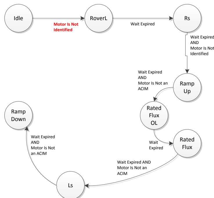
Figure 6-22. Stator Inductance EST State
