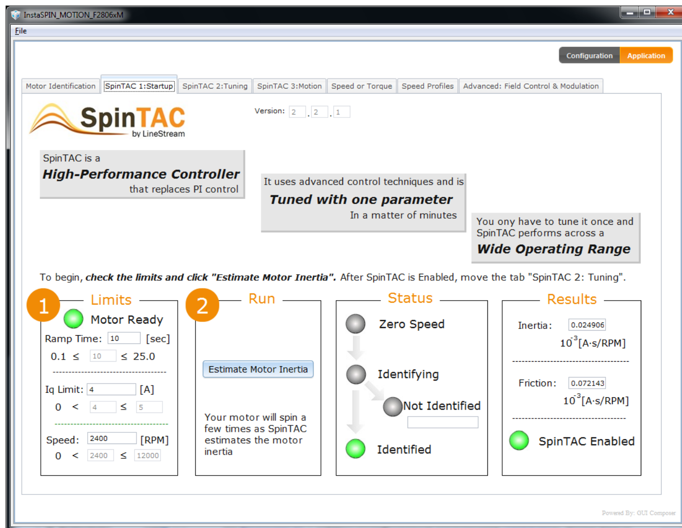
Figure 2-3. InstaSPIN-MOTION GUI Using SpinTAC 1:Startup Tab
