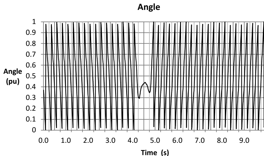
Figure 14-21. Angle Plot
