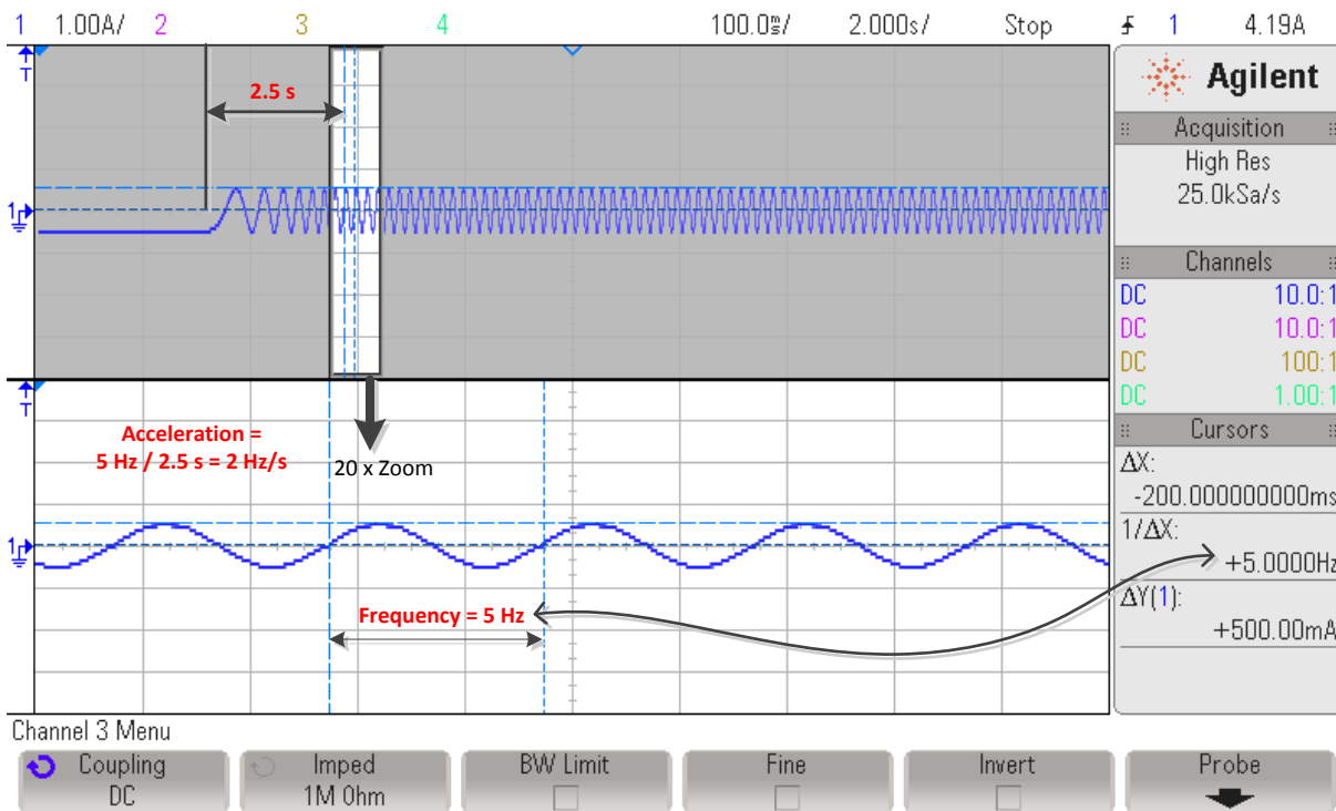
Figure 6-29. Oscilloscope Plot of ACIM RampUp Acceleration
