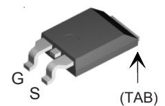
PLUS220 SMD (IXTV...S)
