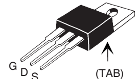
TO-220 (IXTP)
