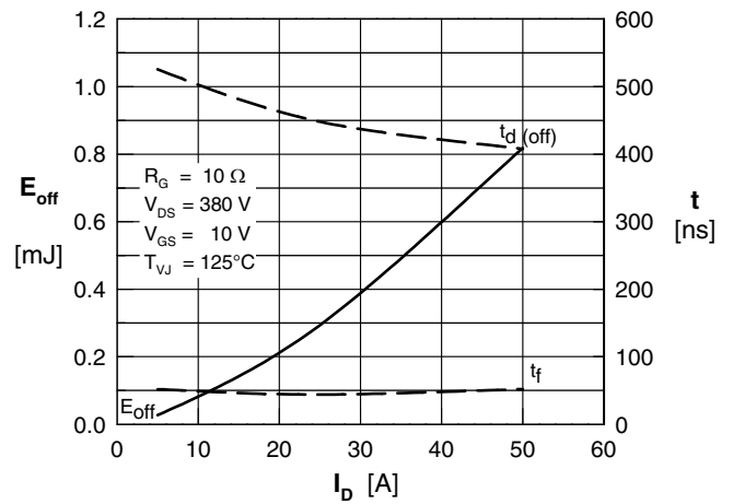
Fig. 14 Typ. turn-off energy & switching times vs. collector current, inductive switching
