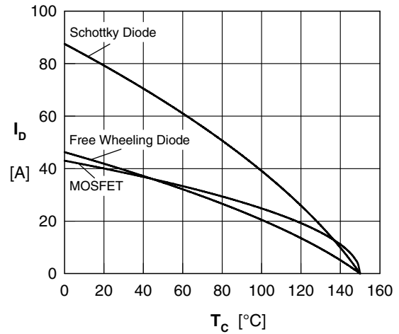
Fig. 12 Drain current I_D vs. case temperature T_c
