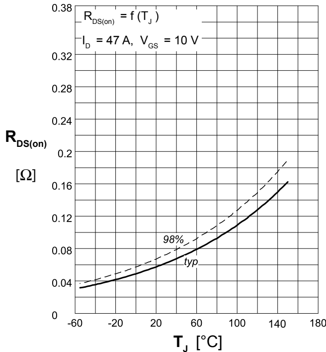
Fig. 9 Drain source on-state resistance R_{DS(on)} versus junction temperature T_J (MOSFET only)
