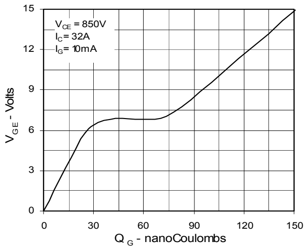
Fig. 11. Gate Charge
