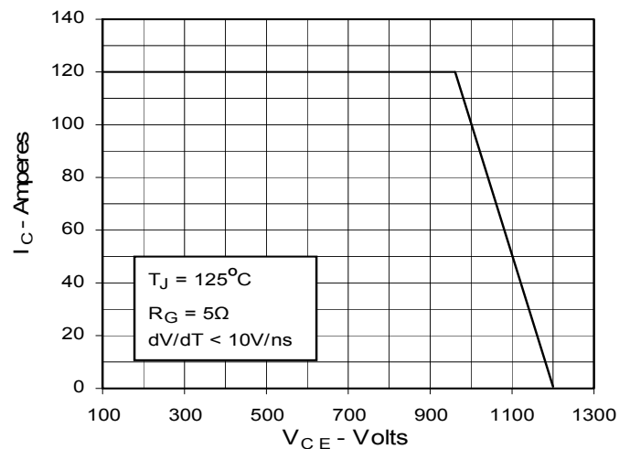
Fig. 16. Reverse-Bias Safe Operating Area
