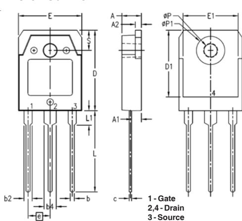
TO-3P Outline
