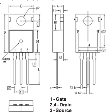
TO-220 Outline
