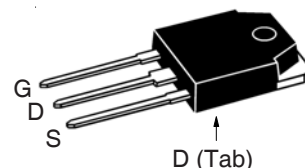
TO-247 (IXFH)
