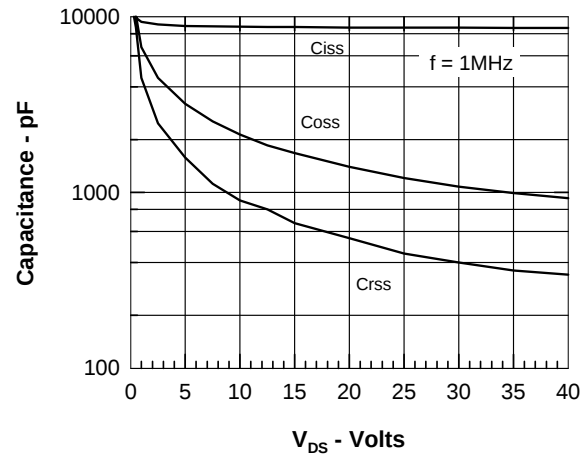
Figure 8. Capacitance Curves
