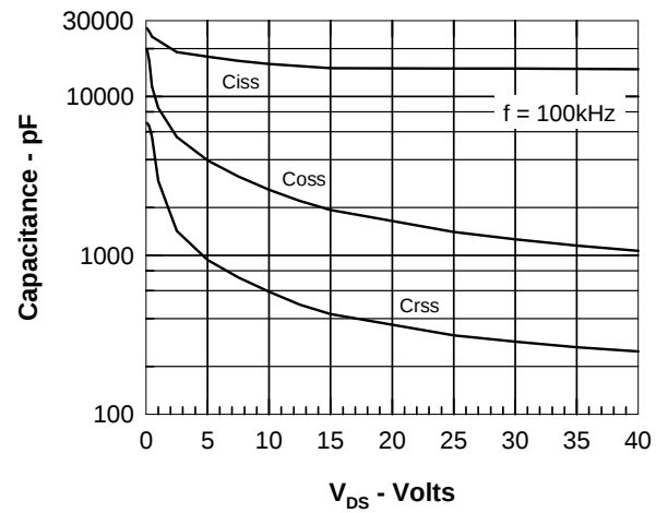
Fig.8 Capacitance Curves
