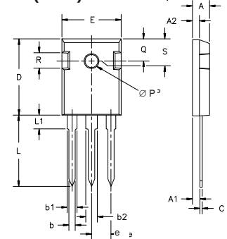
TO-247 (IXFH) Outline
