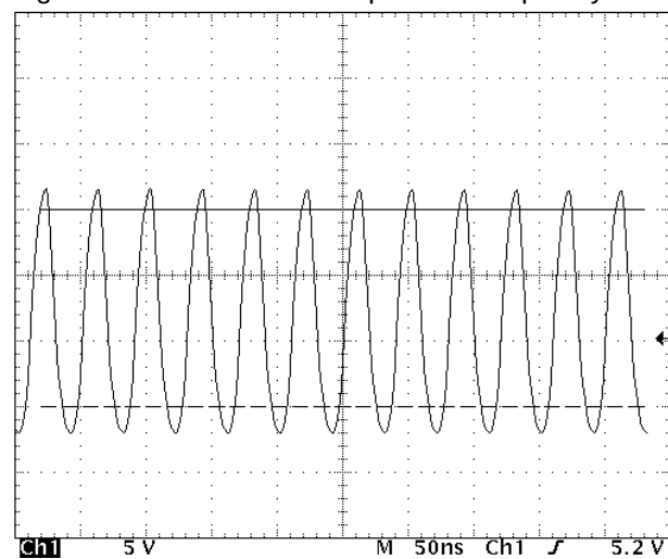
Figure 13 50MHz Burst Repetition Frequency
