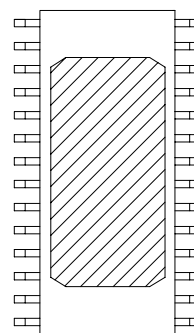
Figure 15: IXDD415SI Bottom Side Heat Sinking Metalization
