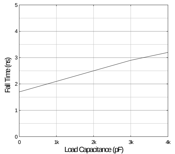
Fig. 4 Fall Time vs. Load Capacitance V_{CC} = 15V , V_{OH} = 12V To 2V
