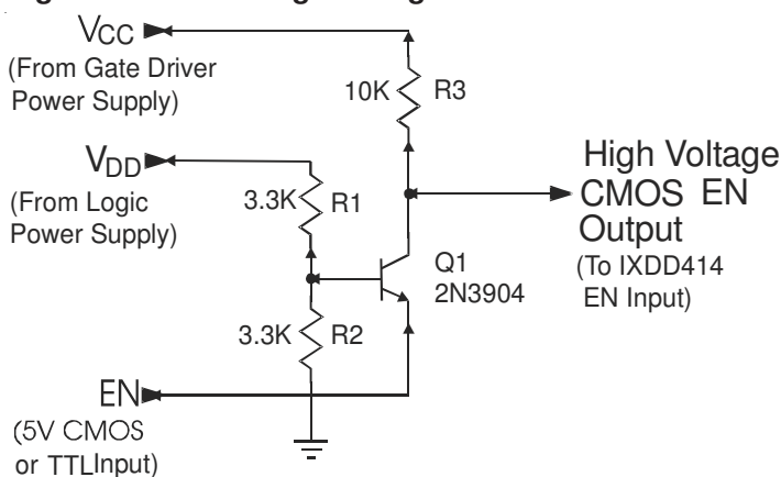
Figure 28 - TTL to High Voltage CMOS Level Translator
