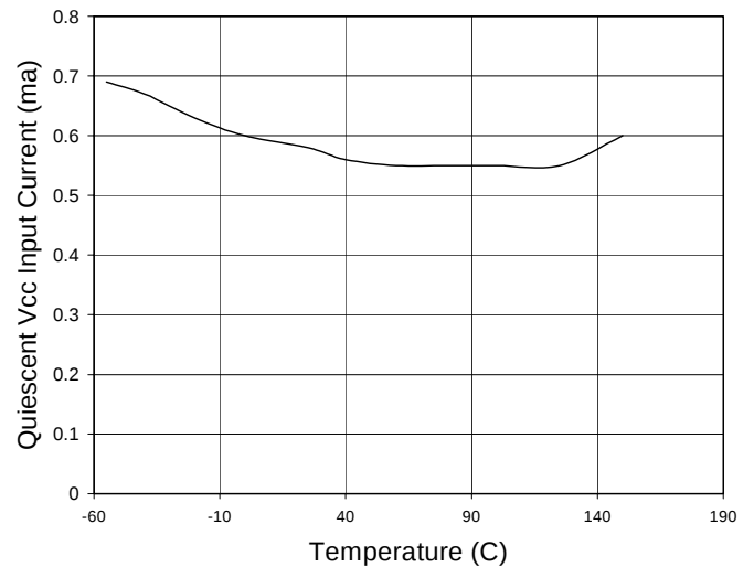
Fig. 22 Quiescent Supply Current vs. Temperature V_{CC} = 18V , V_{in} = 5V@1kHz , CL = 1000\text{ pF}
