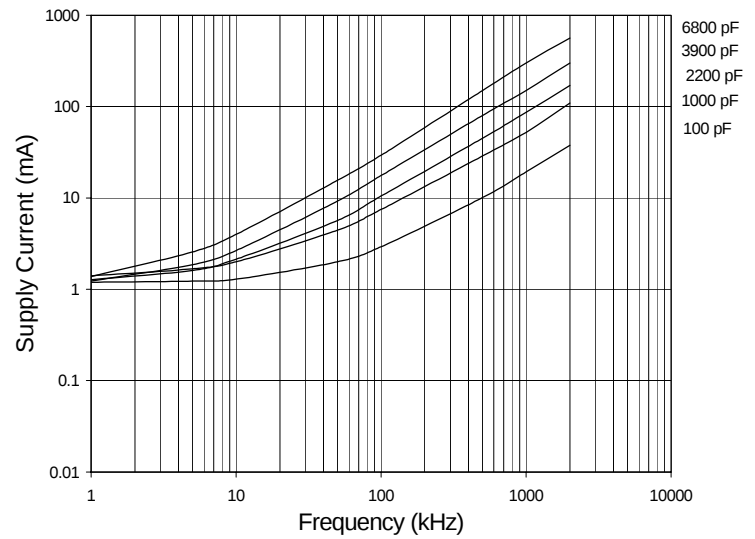
Fig. 18 Supply Current vs. Frequency V_{CC} = 35V
