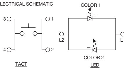
ELECTRICAL SCHEMATIC
