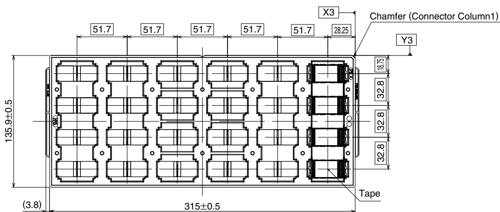
JEDEC Tray for IT3D 200 Position Receptacles
