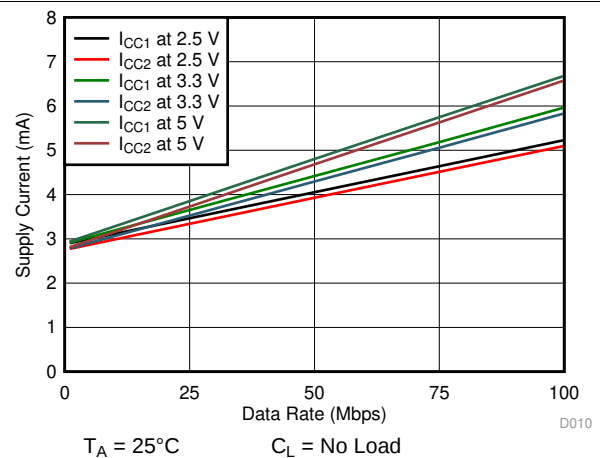
Figure 12. ISO7742-Q1 Supply Current vs Data Rate (With No Load)
