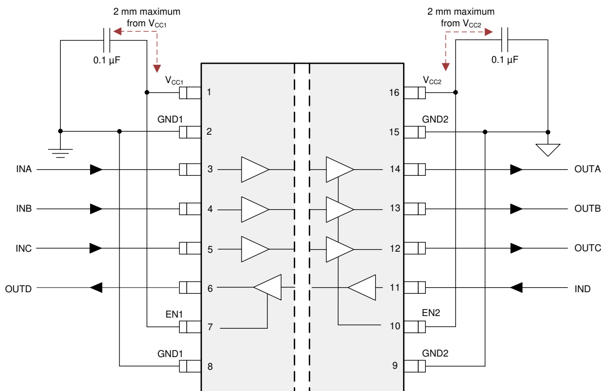
Figure 25. Typical ISO774x-Q1 Circuit Hook-up
