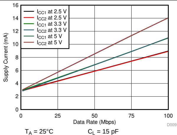
Figure 11. ISO7742-Q1 Supply Current vs Data Rate (With 15-pF Load)
