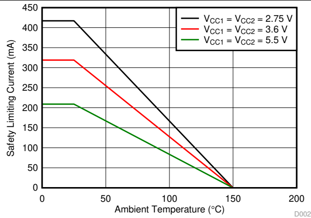
Figure 1. Thermal Derating Curve for Safety Limiting Current for DWW-16 Package
