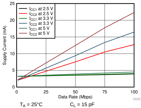
Figure 7. ISO7740-Q1 Supply Current vs Data Rate (With 15-pF Load)
