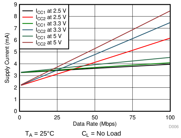
Figure 8. ISO7740-Q1 Supply Current vs Data Rate (With No Load)
