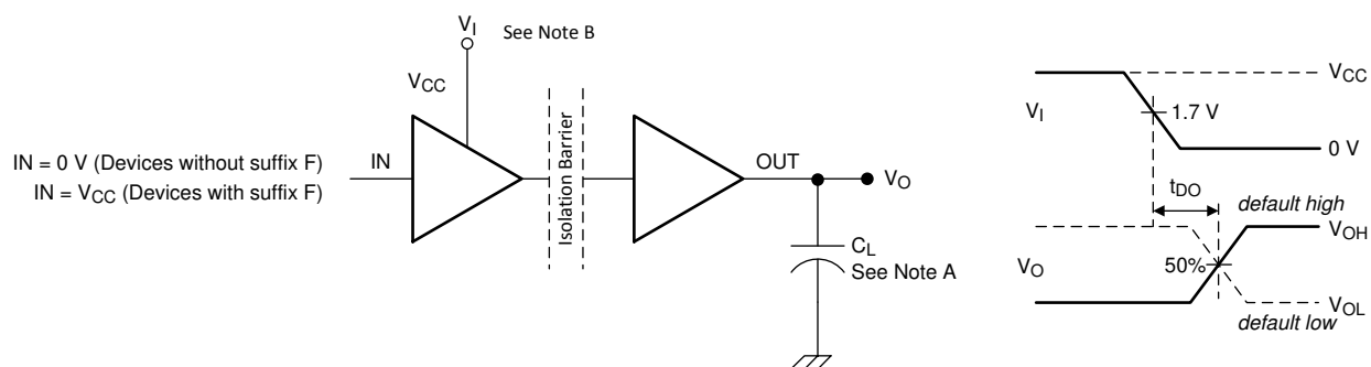
Figure 19. Default Output Delay Time Test Circuit and Voltage Waveforms
