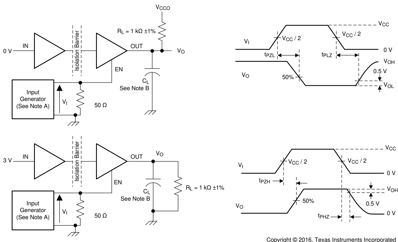
Figure 17. Switching Characteristics Test Circuit and Voltage Waveforms
