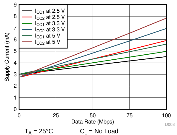
Figure 10. ISO7741-Q1 Supply Current vs Data Rate (With No Load)
