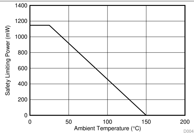
Figure 4. Thermal Derating Curve for Safety Limiting Power for DWW-16 Package
