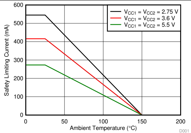
Figure 2. Thermal Derating Curve for Safety Limiting Current for DW-16 Package
