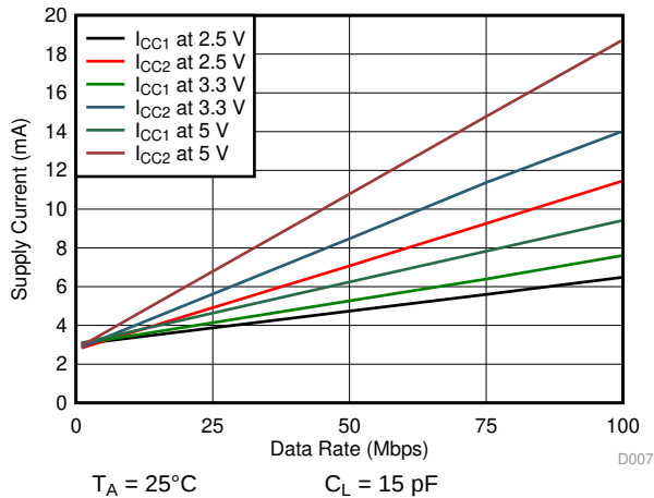
Figure 9. ISO7741-Q1 Supply Current vs Data Rate (With 15-pF Load)
