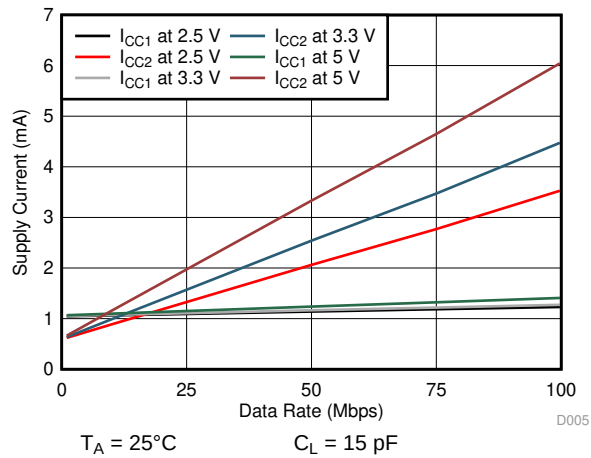
Figure 5. ISO7710-Q1 Supply Current vs Data Rate (With 15 pF Load)
