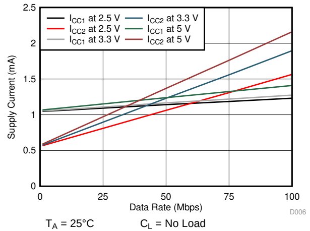
Figure 6. ISO7710-Q1 Supply Current vs Data Rate (With No Load)
