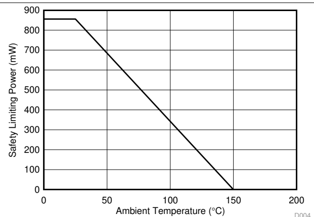
Figure 4. Thermal Derating Curve for Limiting Power per VDE for D-8 Package
