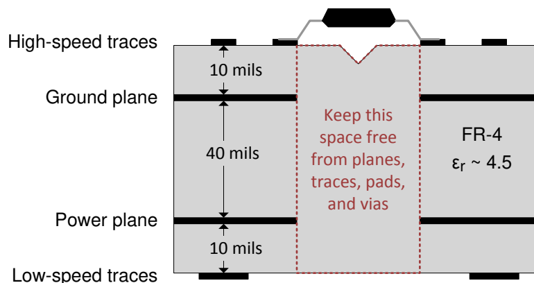
Figure 22. Layout Example
