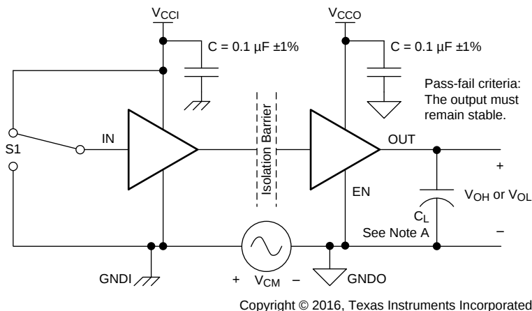
Figure 16. Common-Mode Transient Immunity Test Circuit
