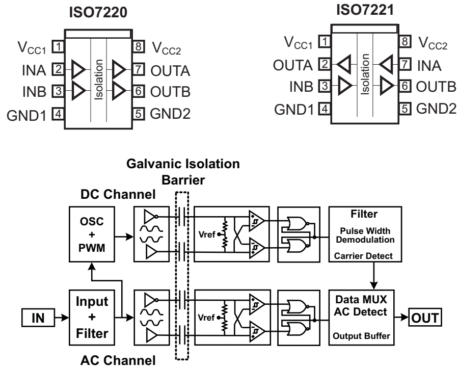
Figure 1. Single-Channel Function Diagram
