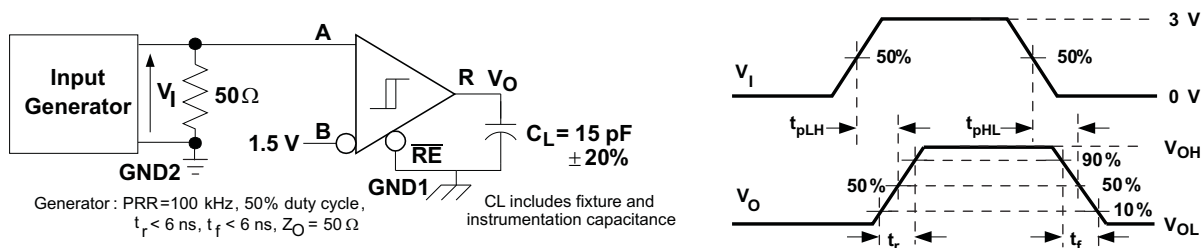
Figure 19. Receiver Switching Test Circuit and Waveforms
