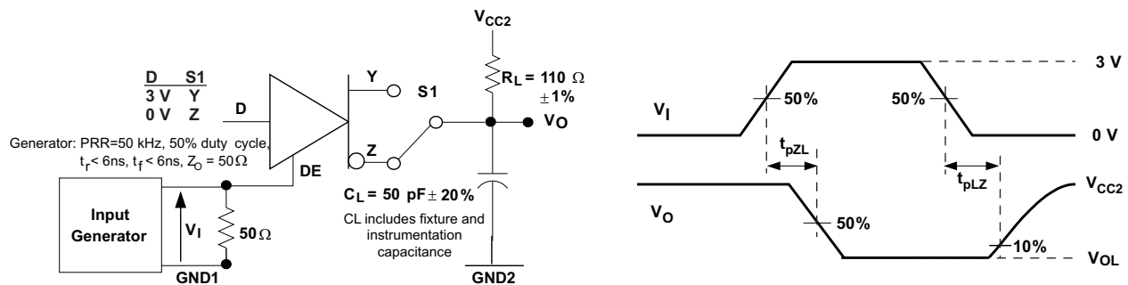
Figure 17. Driver Low-Level Output Enable and Disable Time Test Circuit and Voltage Waveform
