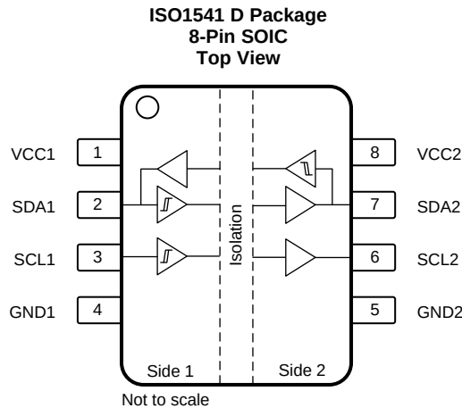
Pin Functions—ISO1541
