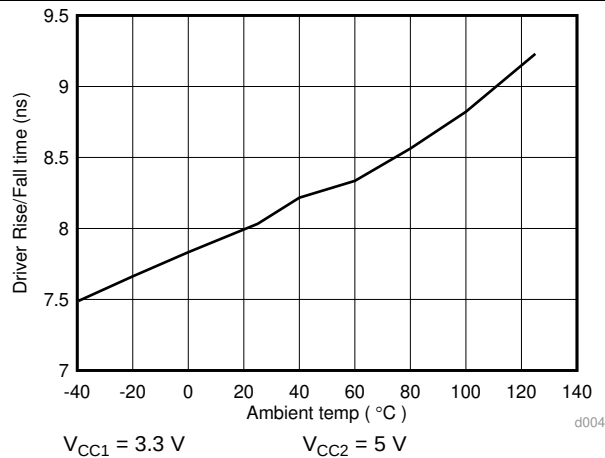
Figure 17. ISO143x Driver Rise/Fall Time (ns) Vs Temperature ( ^\circ\text{C} )
