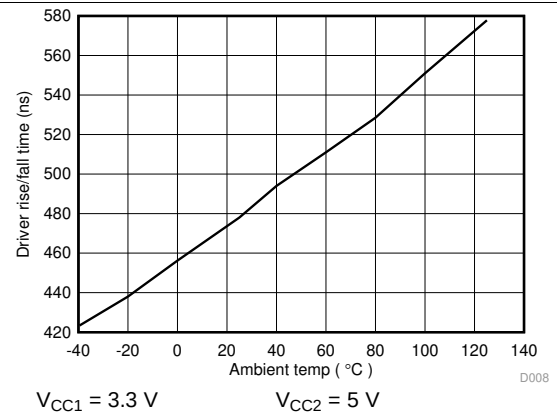
Figure 16. ISO141x Driver Rise/fall Time (ns) Vs Temperature ( ^\circ\text{C} )
