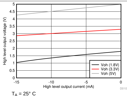
Figure 22. Receiver Buffer High Level Output Voltage Vs High Level Output Current
