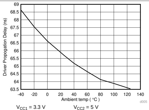
Figure 20. ISO143x Driver Propagation Delay (ns) Vs Temperature ( ^\circ\text{C} )
