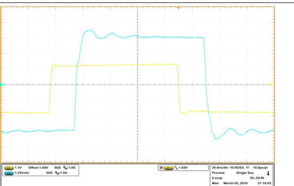
Figure 29. ISO141x Driver Propagation Delay
