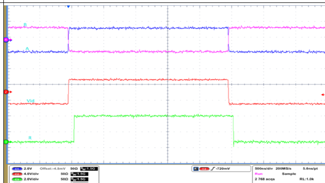
Figure 30. ISO143x Driver Propagation Delay
