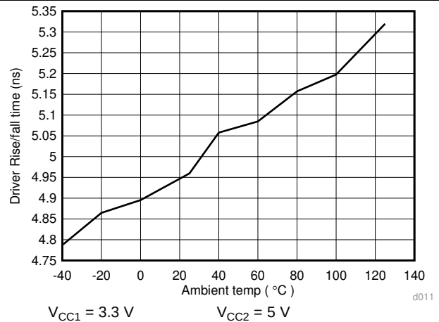
Figure 18. ISO145x Driver Rise/Fall Time (ns) Vs Temperature ( ^\circ\text{C} )
