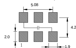
Recommended Pad Layout
