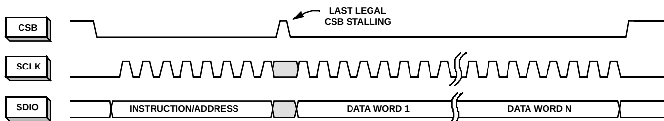
FIGURE 41. N-BYTE TRANSFER
