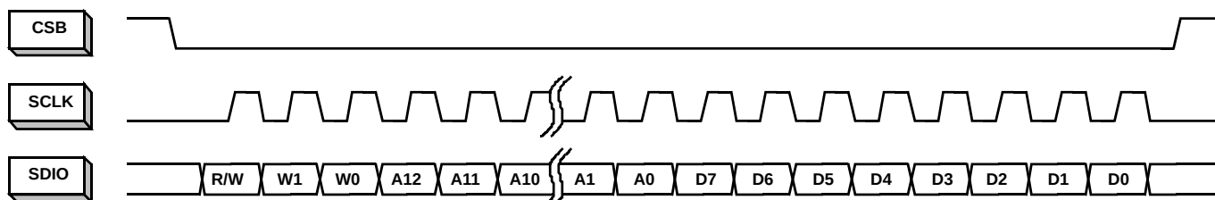
FIGURE 36. MSB-FIRST ADDRESSING
