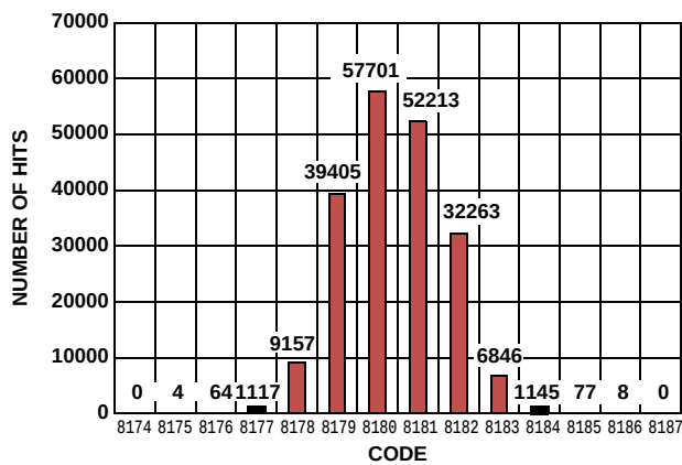
FIGURE 12. NOISE HISTOGRAM
