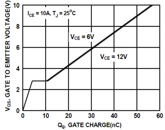
Figure 10. Gate Charge
