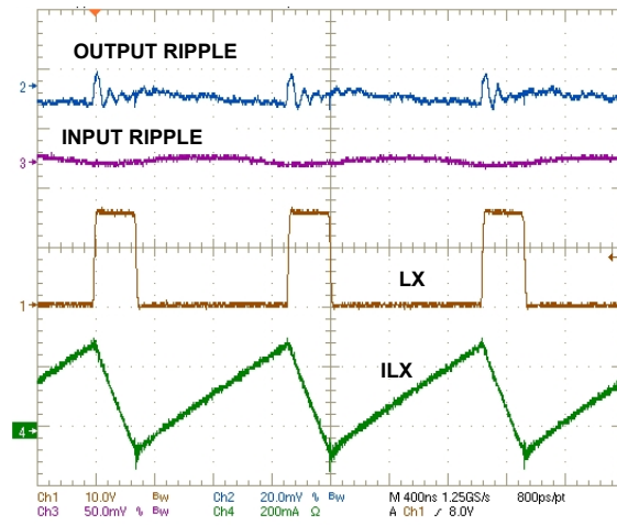
FIGURE 8. STEADY STATE OPERATION (INDUCTOR CONTINUOUS CONDUCTION), V_{IN} = 3.3V , V_O = 15V , I_O = 30mA
