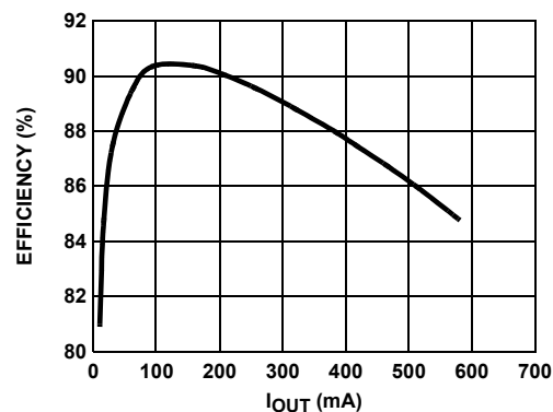
FIGURE 2. EFFICIENCY vs I_{OUT} , V_{IN} = 3.3V , V_O = 5V
