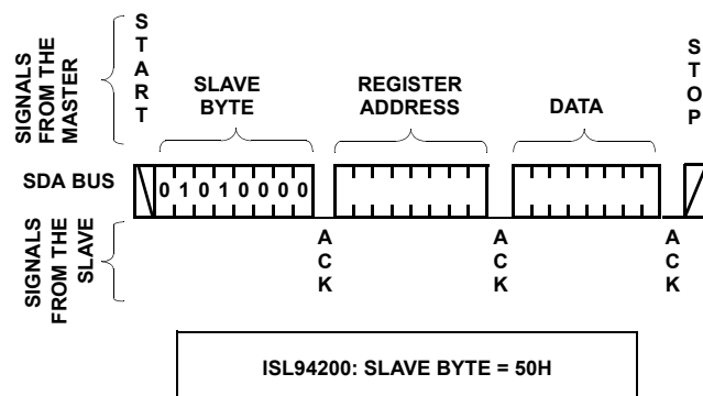
FIGURE 11. WRITE SEQUENCE
