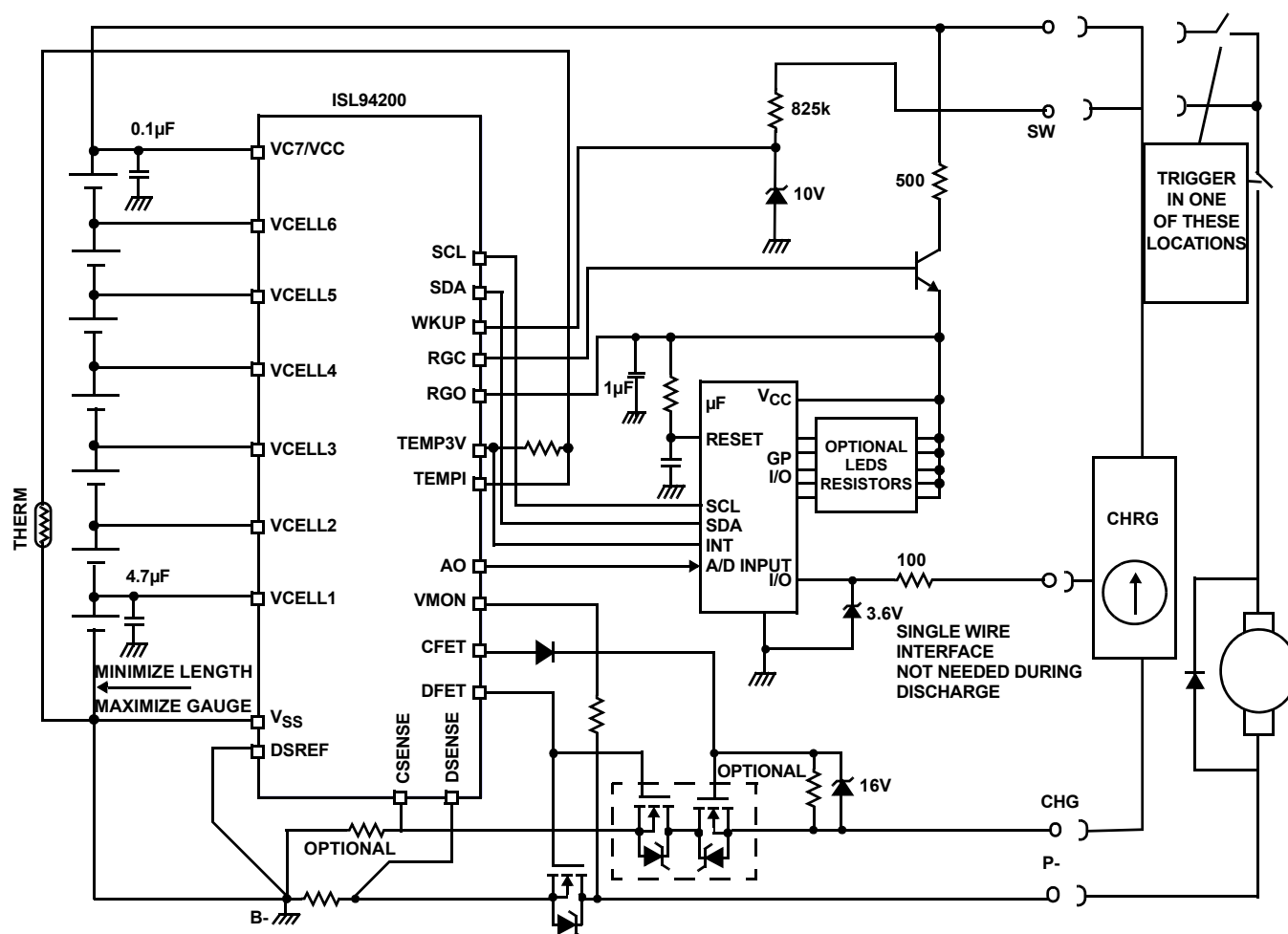
FIGURE 16. 7-CELL APPLICATION CIRCUIT WITH SWITCH WAKE-UP AND SEPARATE CHARGE/DISCHARGE
