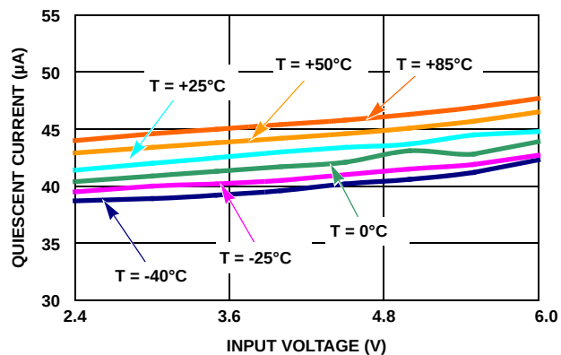
FIGURE 1. QUIESCIENT CURRENT vs INPUT VOLTAGE ( V_{OUT1} = 2.1V , ONLY LDO1 ENABLED)
