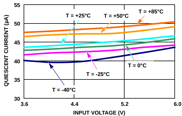
FIGURE 5. QUIESCIENT CURRENT vs INPUT VOLTAGE ( V_{OUT2} = 3.3V , ONLY LDO2 ENABLED)
