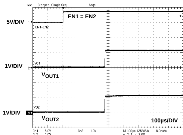
FIGURE 11. ENABLE OPERATION ( V_{IN} = 3.6V , V_{OUT1} = V_{OUT2} = 1.2V )
