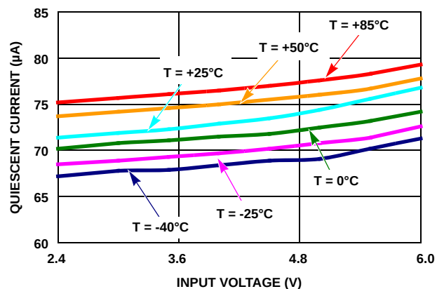
FIGURE 3. QUIESCIENT CURRENT vs INPUT VOLTAGE ( V_{OUT1} = V_{OUT2} = 2.1V , LDO1 AND LDO2 ENABLED)
