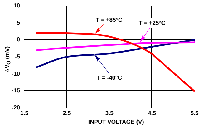
FIGURE 8. \Delta V_{OUT} vs INPUT VOLTAGE ( V_{OUT\_NOMINAL} = 1.2V , I_{OUT} = 150mA )
