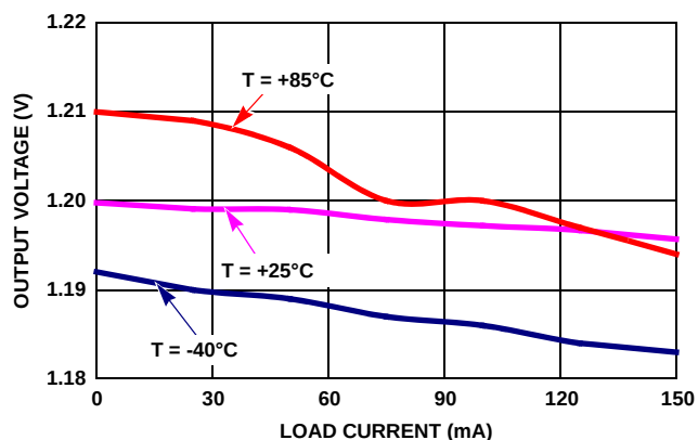
FIGURE 9. LOAD REGULATION ( V_{IN} = 1.8V , V_{OUT} = 1.2V )
