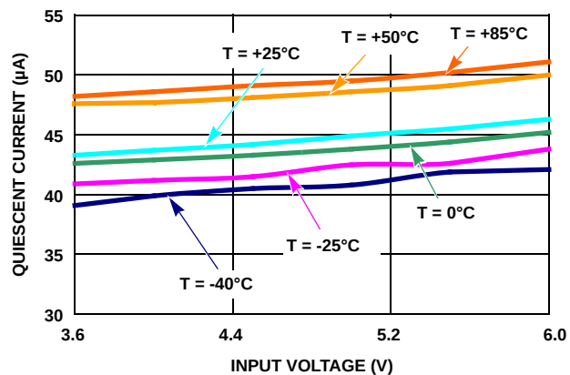
FIGURE 4. QUIESCIENT CURRENT vs INPUT VOLTAGE ( V_{OUT1} = 3.3V , ONLY LDO1 ENABLED)
