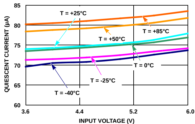
FIGURE 6. QUIESCIENT CURRENT vs INPUT VOLTAGE ( V_{OUT1} = V_{OUT2} = 3.3V , LDO1 AND LDO2 ENABLED)
