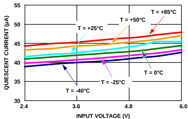
FIGURE 2. QUIESCIENT CURRENT vs INPUT VOLTAGE ( V_{OUT2} = 2.1V , ONLY LDO2 ENABLED)
