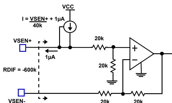
FIGURE 32. EQUIVALENT DIFFERENTIAL AMPLIFIER
