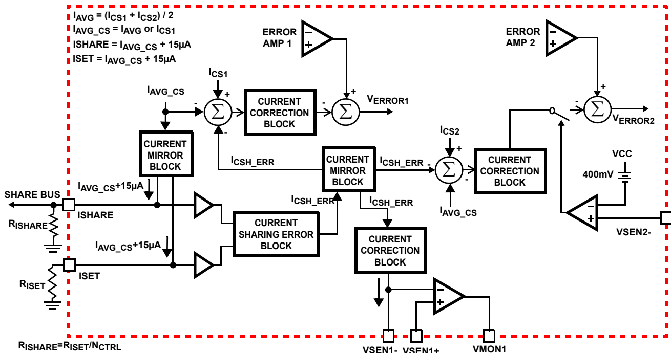
FIGURE 24. SIMPLIFIED CURRENT SHARE AND INTERNAL BALANCE IMPLEMENTATION
