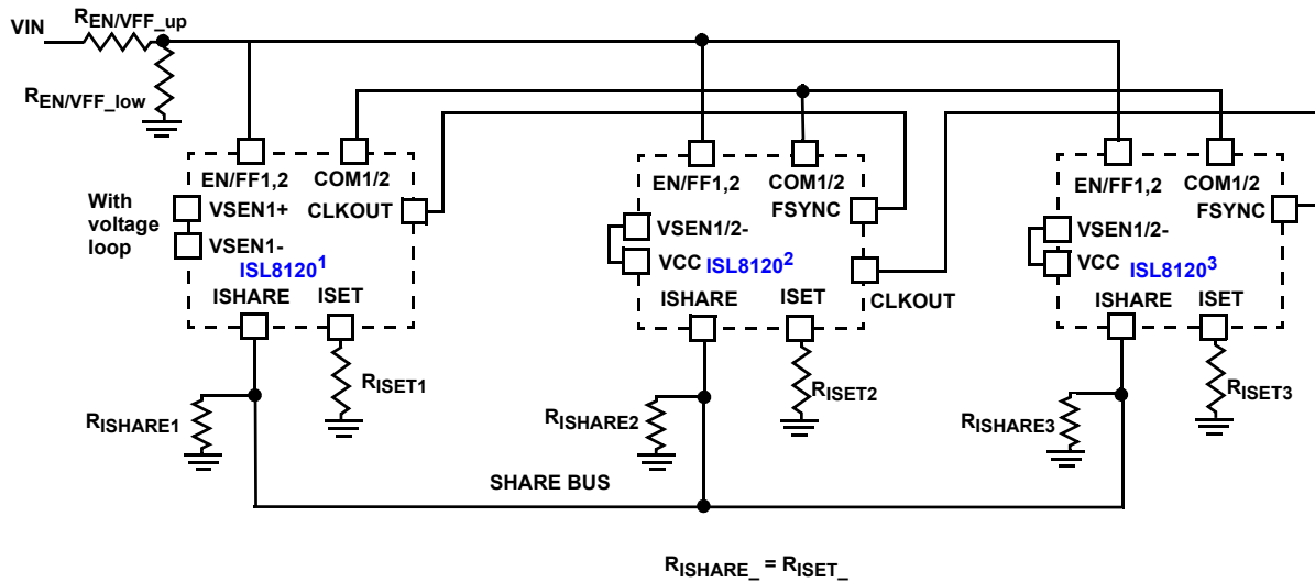
FIGURE 25. SIMPLIFIED 6-PHASE SINGLE OUTPUT IMPLEMENTATION
