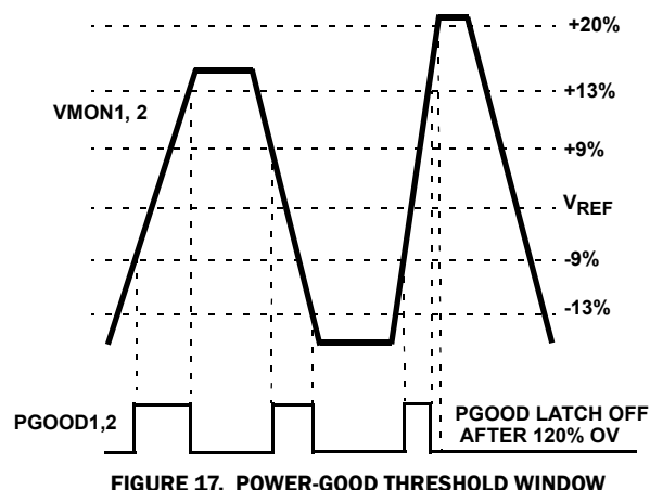
FIGURE 17. POWER-GOOD THRESHOLD WINDOW
