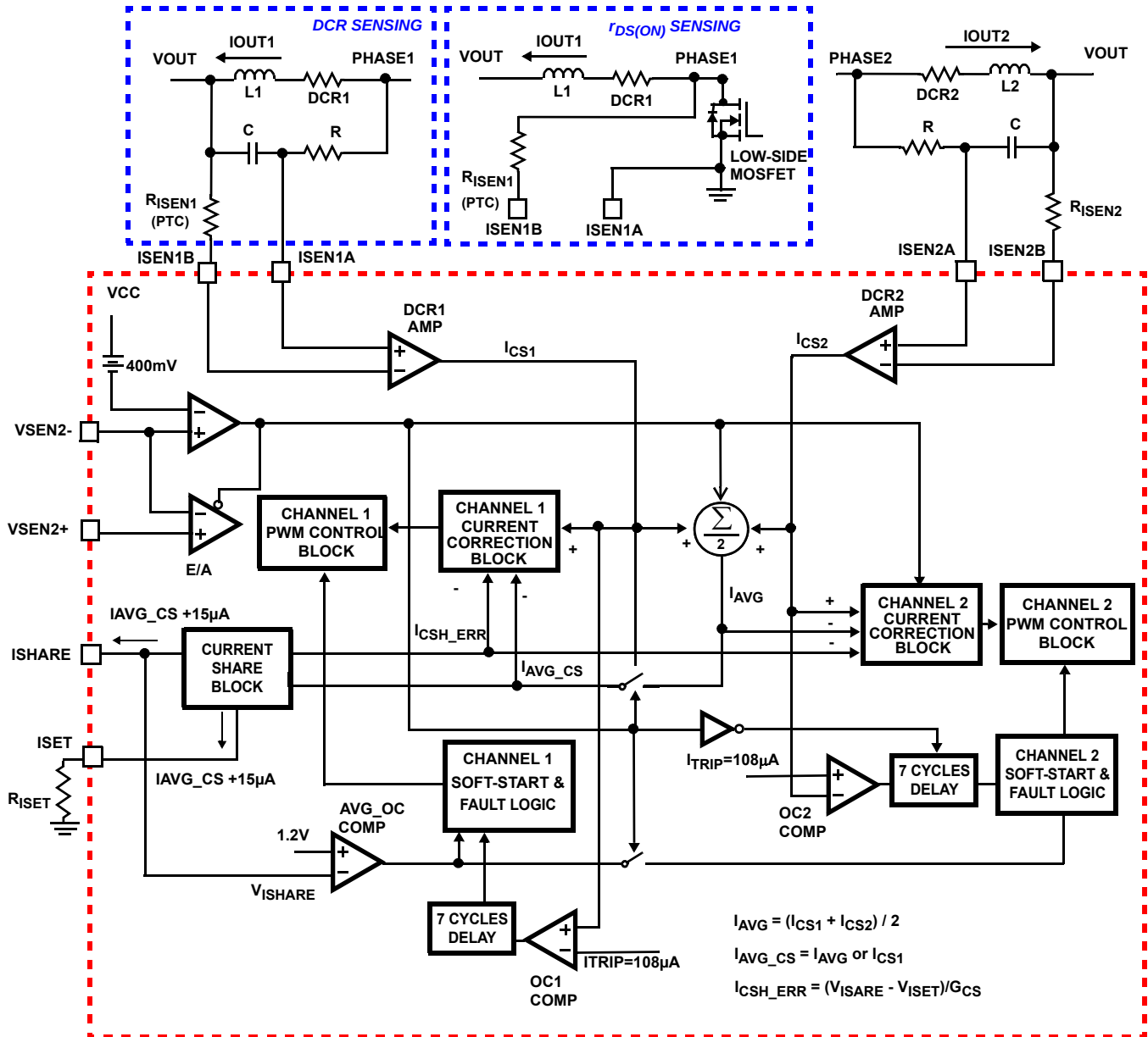
FIGURE 23. SIMPLIFIED CURRENT SAMPLING AND OVERCURRENT PROTECTION
