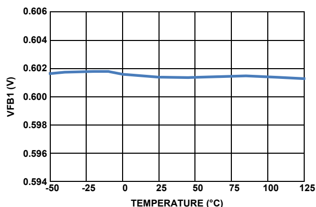
FIGURE 2. CHANNEL 1 ACCURACY vs TEMPERATURE
