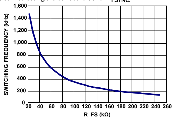
FIGURE 30. R_{FS} vs SWITCHING FREQUENCY
