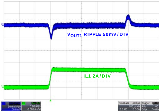
FIGURE 37. LOAD TRANSIENT CHANNEL 1
