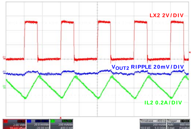
FIGURE 34. STEADY STATE OPERATION AT NO LOAD CHANNEL 2
