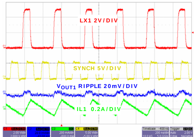
FIGURE 23. CHANNEL 1 STEADY STATE OPERATION AT NO LOAD WITH FREQUENCY = 6MHz
