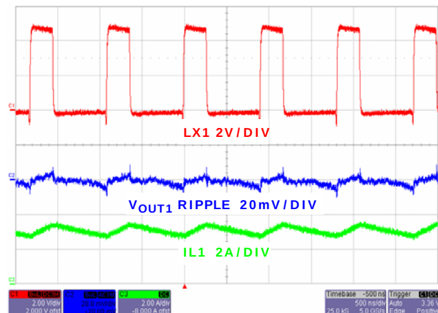
FIGURE 12. STEADY STATE OPERATION WITH FULL LOAD CHANNEL 1
