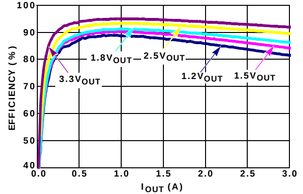
FIGURE 3. EFFICIENCY, T_A = +25^\circ\text{C} , V_{IN} = 5\text{V}
