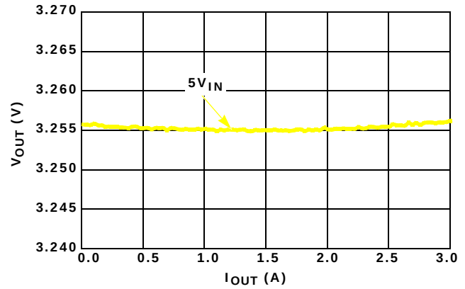
FIGURE 9. LOAD REGULATION, V_{OUT} = 3.3\text{V} T_A = +25^\circ\text{C}
