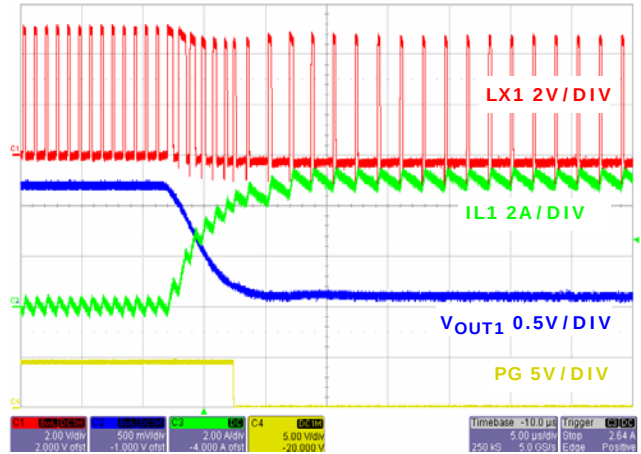
FIGURE 27. OUTPUT SHORT CIRCUIT CHANNEL 1
