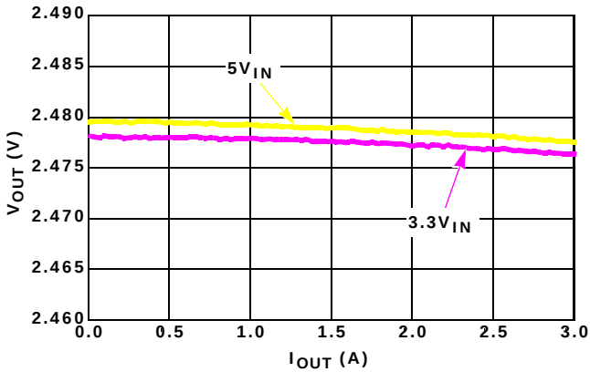
FIGURE 8. LOAD REGULATION, V_{OUT} = 2.5\text{V} T_A = +25^\circ\text{C}
