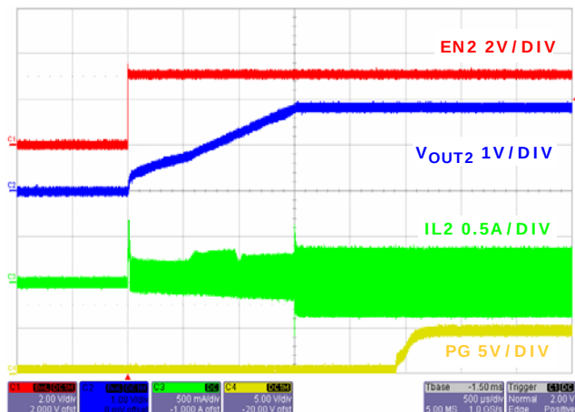
FIGURE 18. SOFT-START WITH NO LOAD CHANNEL 2
