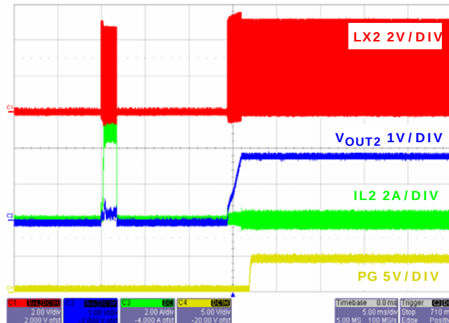
FIGURE 30. OUTPUT SHORT CIRCUIT RECOVERY CHANNEL 2
