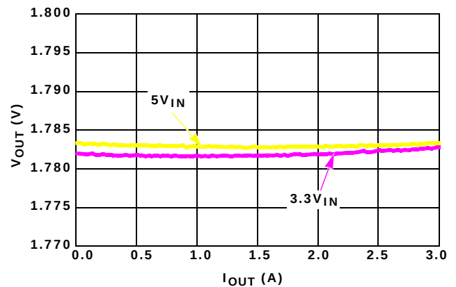
FIGURE 7. LOAD REGULATION, V_{OUT} = 1.8\text{V} T_A = +25^\circ\text{C}
