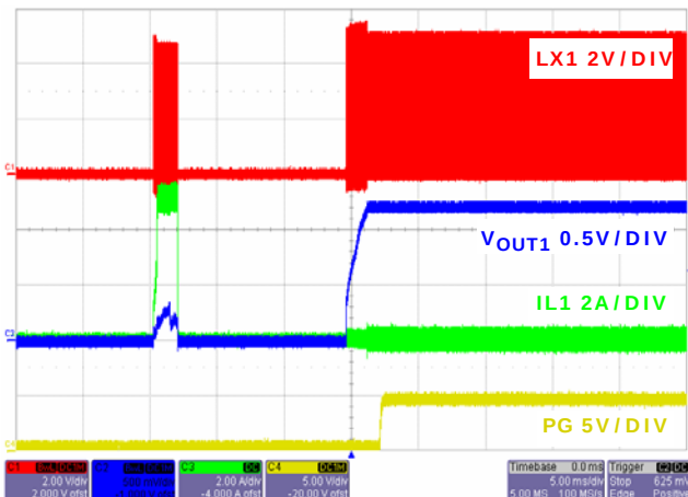
FIGURE 28. OUTPUT SHORT CIRCUIT RECOVERY CHANNEL 1
