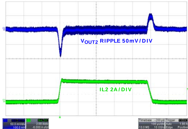
FIGURE 38. LOAD TRANSIENT CHANNEL 2
