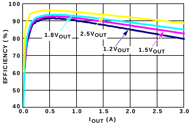
FIGURE 2. EFFICIENCY, T_A = +25^\circ\text{C} , V_{IN} = 3.3\text{V}
