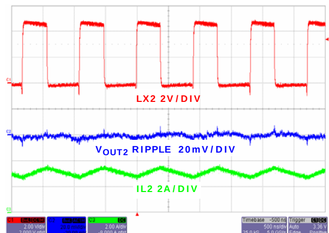
FIGURE 13. STEADY STATE OPERATION WITH FULL LOAD CHANNEL 2
