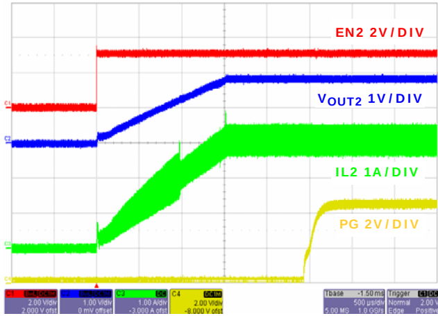
FIGURE 20. SOFT-START AT FULL LOAD CHANNEL 2
