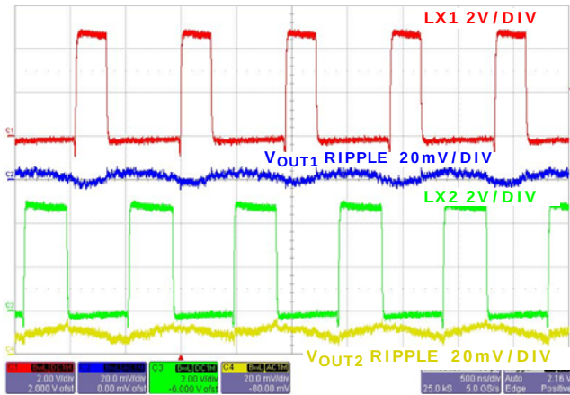
FIGURE 14. STEADY STATE OPERATION WITH FULL LOADS AT BOTH CHANNELS
