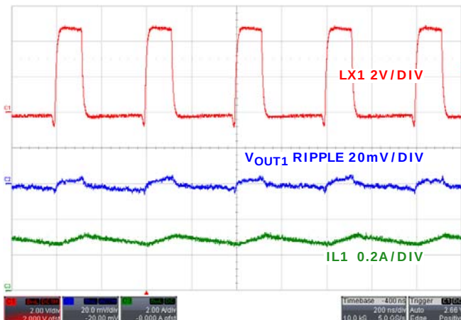
FIGURE 35. STEADY STATE OPERATION WITH FULL LOAD CHANNEL 1
