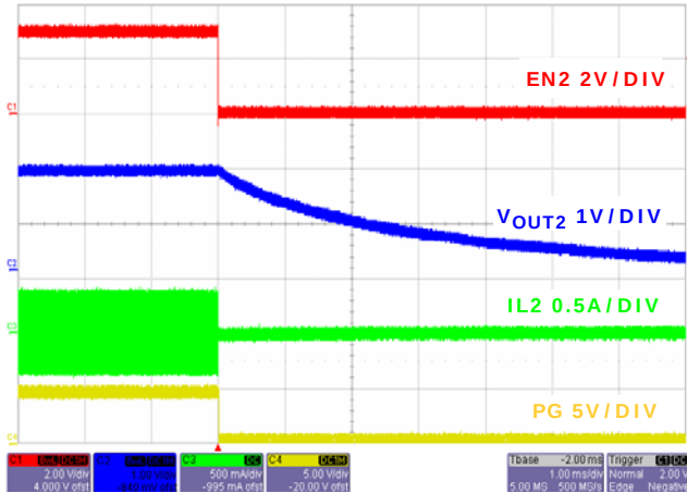
FIGURE 22. SOFT-DISCHARGE SHUTDOWN CHANNEL 2
