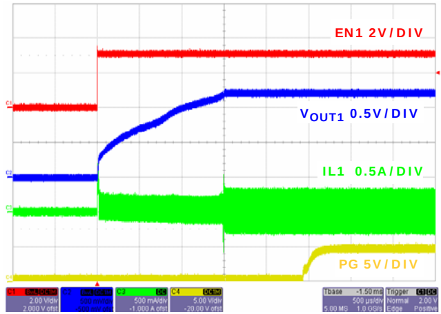
FIGURE 17. SOFT-START WITH NO LOAD CHANNEL 1
