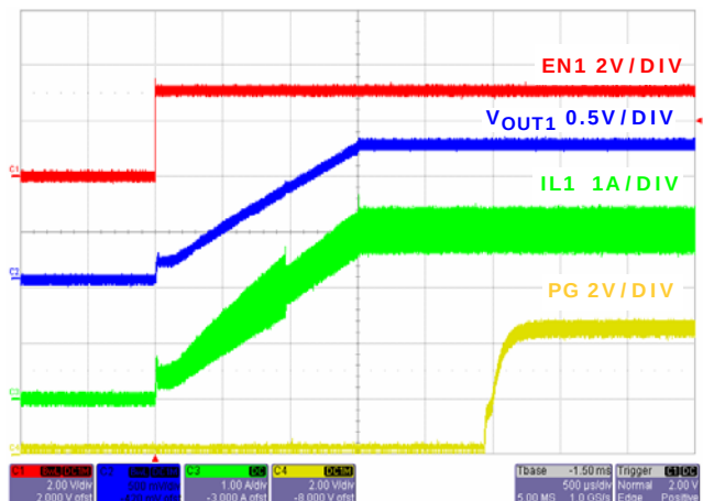
FIGURE 19. SOFT-START AT FULL LOAD CHANNEL 1
