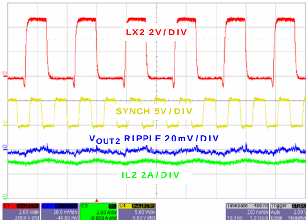
FIGURE 26. CHANNEL 2 STEADY STATE OPERATION AT FULL LOAD WITH FREQUENCY = 6 MHz
