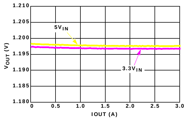
FIGURE 5. LOAD REGULATION, V_{OUT} = 1.2\text{V} T_A = +25^\circ\text{C}
