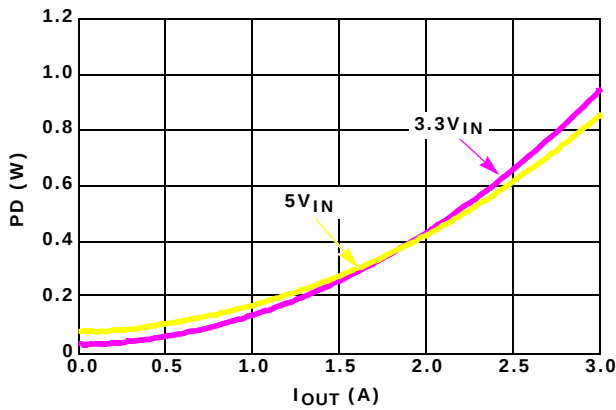
FIGURE 4. POWER DISSIPATION, T_A = +25^\circ\text{C} V_{OUT} = 1.8\text{V}
