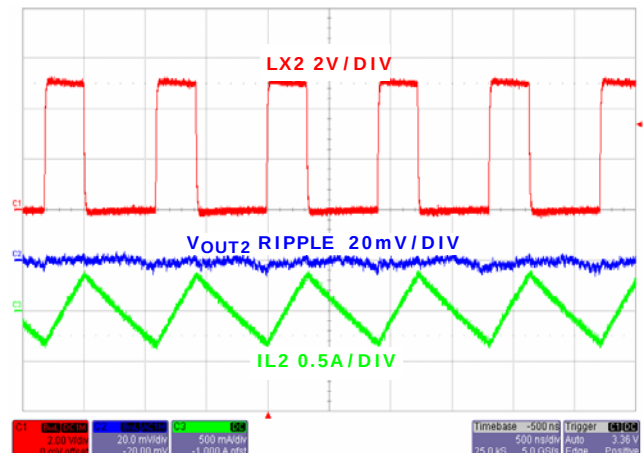
FIGURE 11. STEADY STATE OPERATION AT NO LOAD CHANNEL 2 (PWM)
