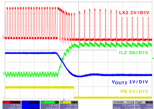
FIGURE 29. OUTPUT SHORT CIRCUIT CHANNEL 2
