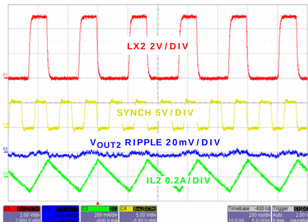
FIGURE 24. CHANNEL 2 STEADY STATE OPERATION AT NO LOAD WITH FREQUENCY = 6MHz
