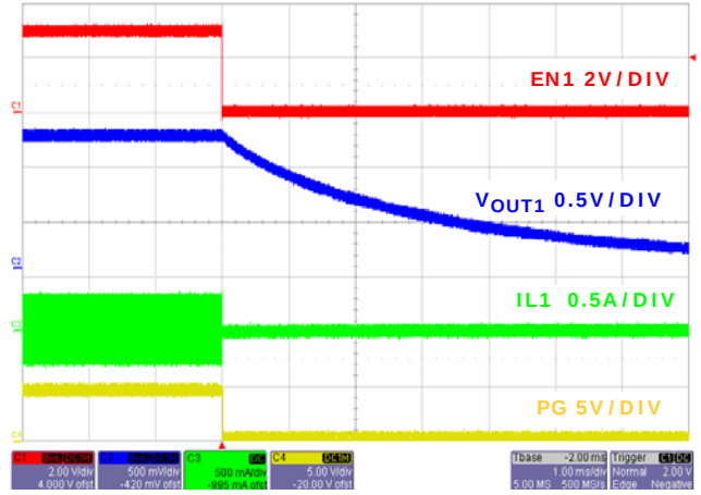
FIGURE 21. SOFT-DISCHARGE SHUTDOWN CHANNEL 1
