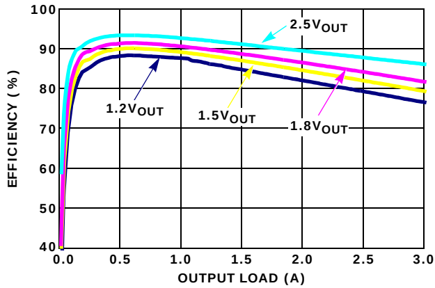
FIGURE 31. EFFICIENCY vs LOAD, 1MHz 3.3V IN DUAL CH1 +25°C
