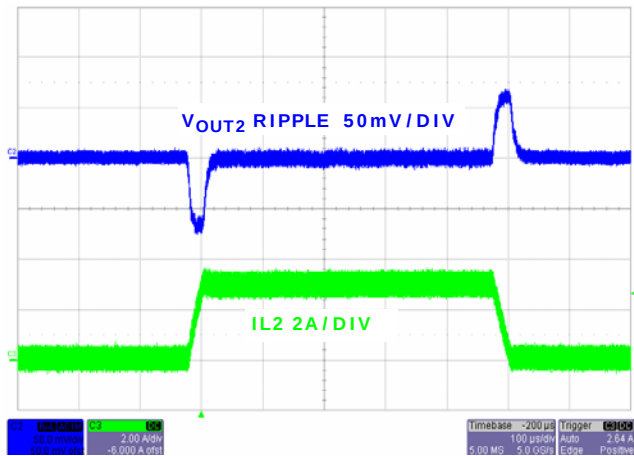
FIGURE 16. LOAD TRANSIENT CHANNEL 2 (PWM)
