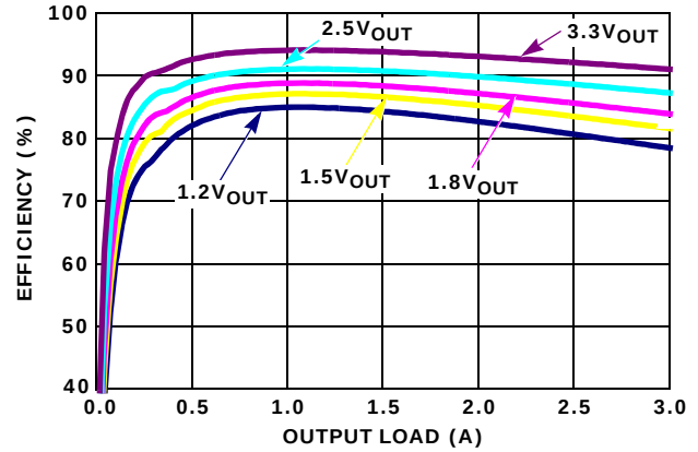
FIGURE 32. EFFICIENCY vs LOAD, 1MHz 5V IN , DUAL CH1 +25°C
