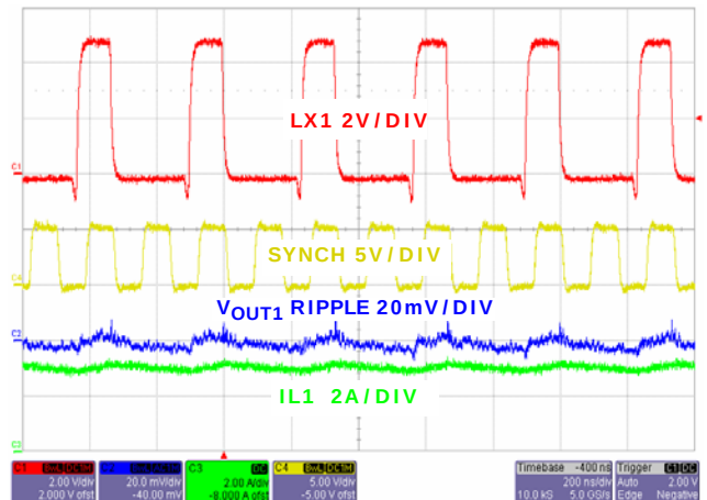
FIGURE 25. CHANNEL 1 STEADY STATE OPERATION AT FULL LOAD WITH FREQUENCY = 6MHz
