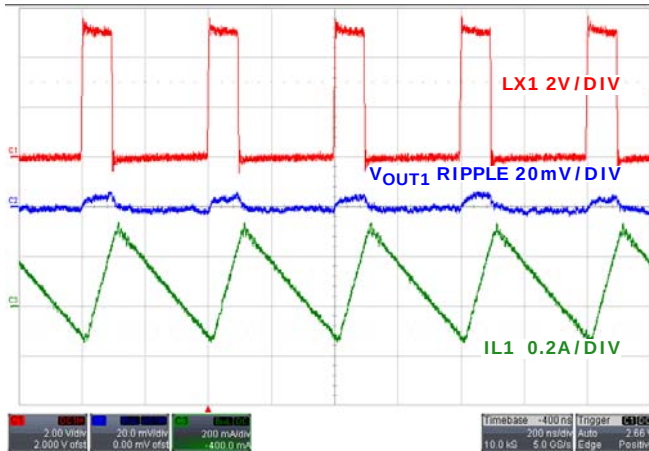
FIGURE 33. STEADY STATE OPERATION AT NO LOAD CHANNEL 1
