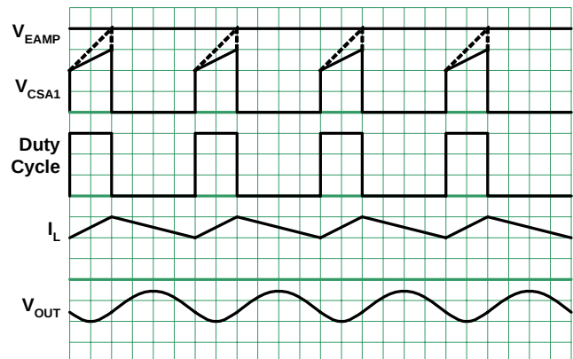
FIGURE 39. PWM OPERATION WAVEFORMS
