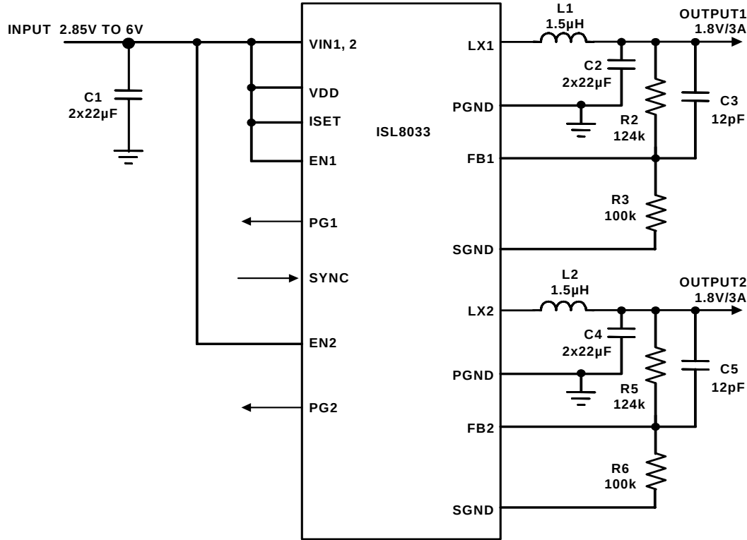
FIGURE 1. TYPICAL APPLICATION DIAGRAM - DUAL INDEPENDENT OUTPUTS
