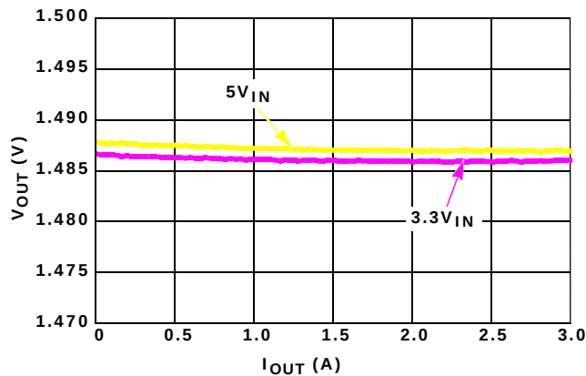
FIGURE 6. LOAD REGULATION, V_{OUT} = 1.5\text{V} T_A = +25^\circ\text{C}
