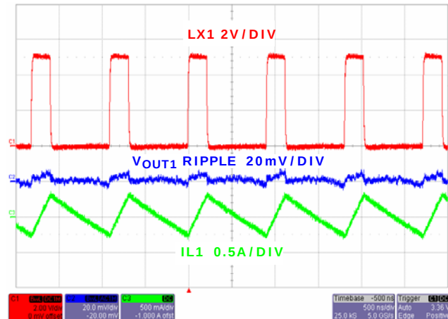
FIGURE 10. STEADY STATE OPERATION AT NO LOAD CHANNEL 1 (PWM)
