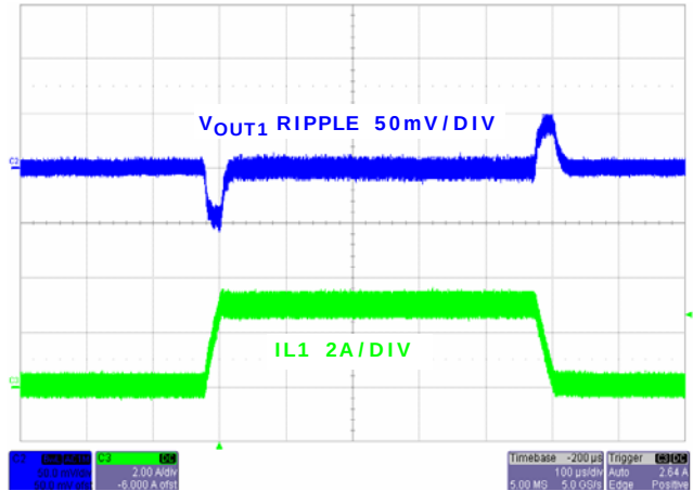
FIGURE 15. LOAD TRANSIENT CHANNEL 1 (PWM)
