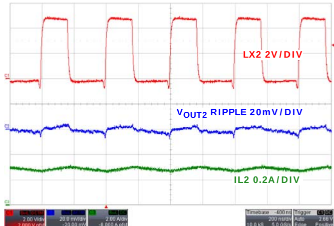
FIGURE 36. STEADY STATE OPERATION WITH FULL LOAD CHANNEL 2
