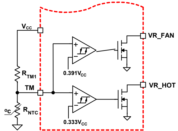
FIGURE 16. BLOCK DIAGRAM OF THERMAL MONITORING FUNCTION
