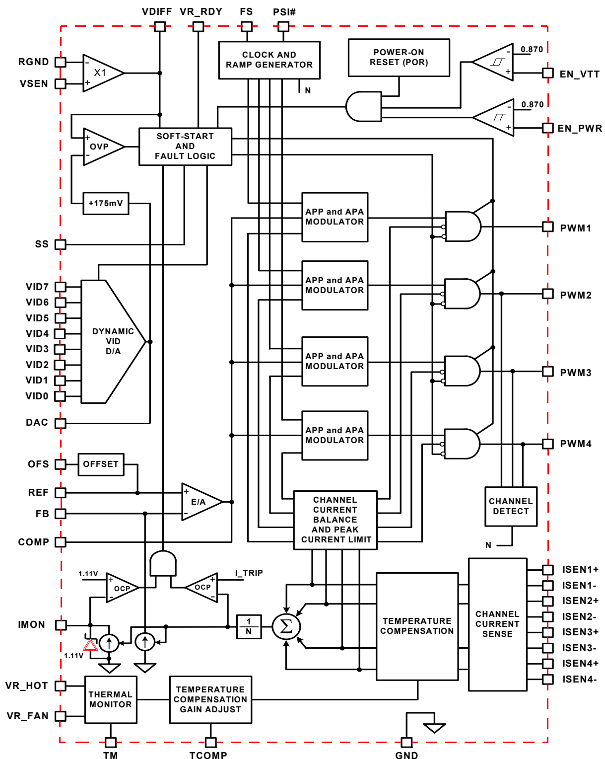
FIGURE 1. BLOCK DIAGRAM
