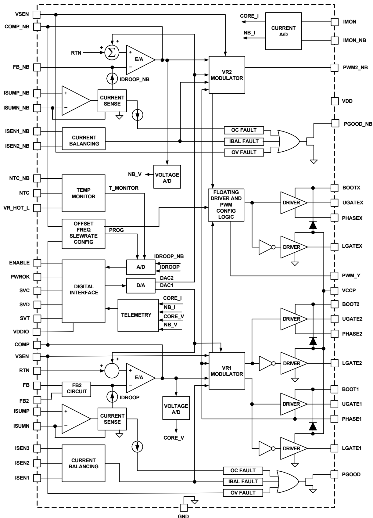
FIGURE 7. BLOCK DIAGRAM
