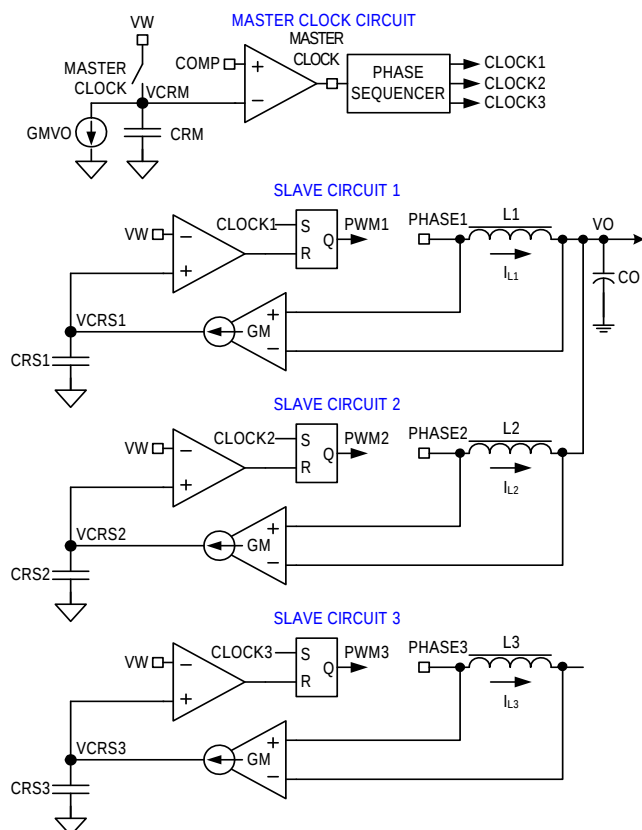
FIGURE 9. R3™ MODULATOR CIRCUIT
