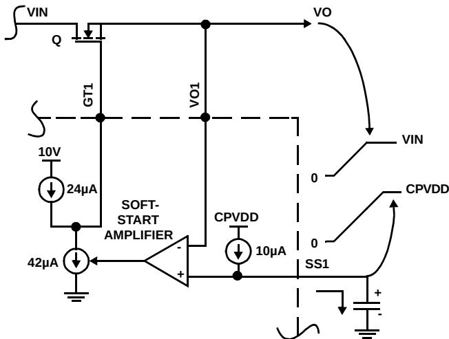
FIGURE 15. SOFT-START OPERATION
