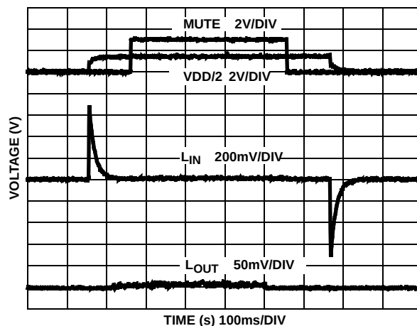
FIGURE 29. 1k\Omega AC-COUPLED CLICK/POP REDUCTION
