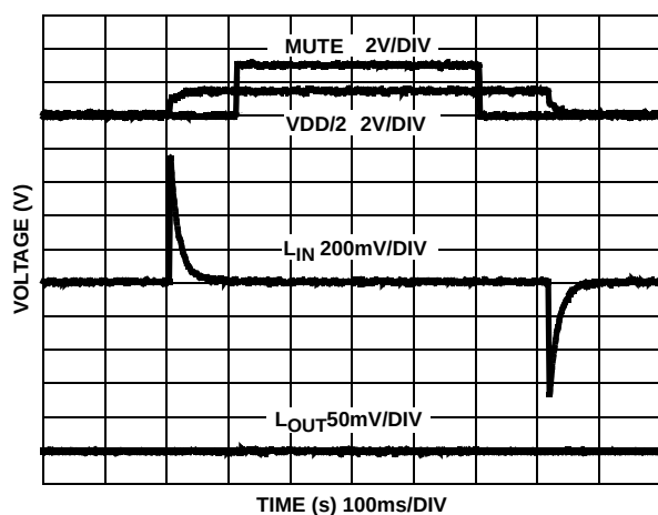
FIGURE 28. 32\Omega AC-COUPLED CLICK/POP REDUCTION
