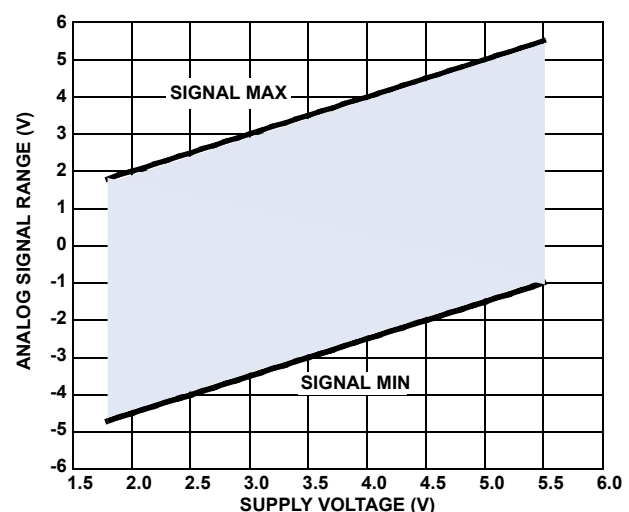
FIGURE 13. ANALOG SIGNAL RANGE vs SUPPLY VOLTAGE
