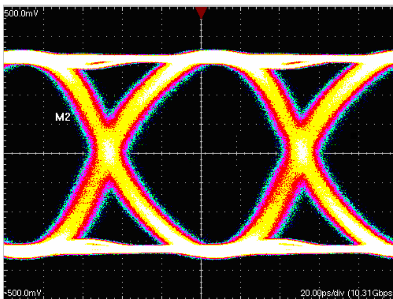
FIGURE 2. ISL36411 10.3125Gb/s OUTPUT FOR A 10M 28AWG CABLE
